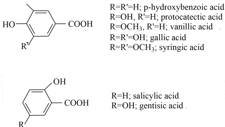
Figure 1. Chemical compounds of basic benzoic acid derivatives.
