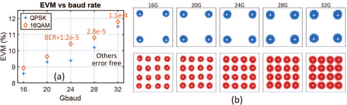
Figure 6. Coherent transmission results of low-cost DP-QPSK and DP-16QAM systems, for one-bit and two-bit digitization, respectively. (a) Error vector magnitude (EVM) vs. baud rate. (b) Constellations of QPSK and 16QAM at each baud rate.
