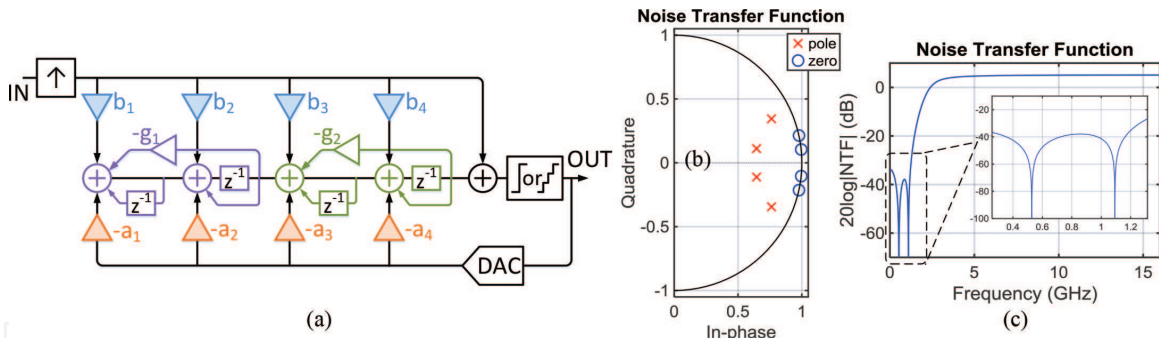
Figure 5. Implementation of 32 GSa/s delta-sigma ADC. (a) Z-domain block diagram of a fourth-order cascade resonator feedback (CRFB) structure. (b) Zeroes and poles of the noise transfer function (NTF). (c) Frequency response of the NTF.
