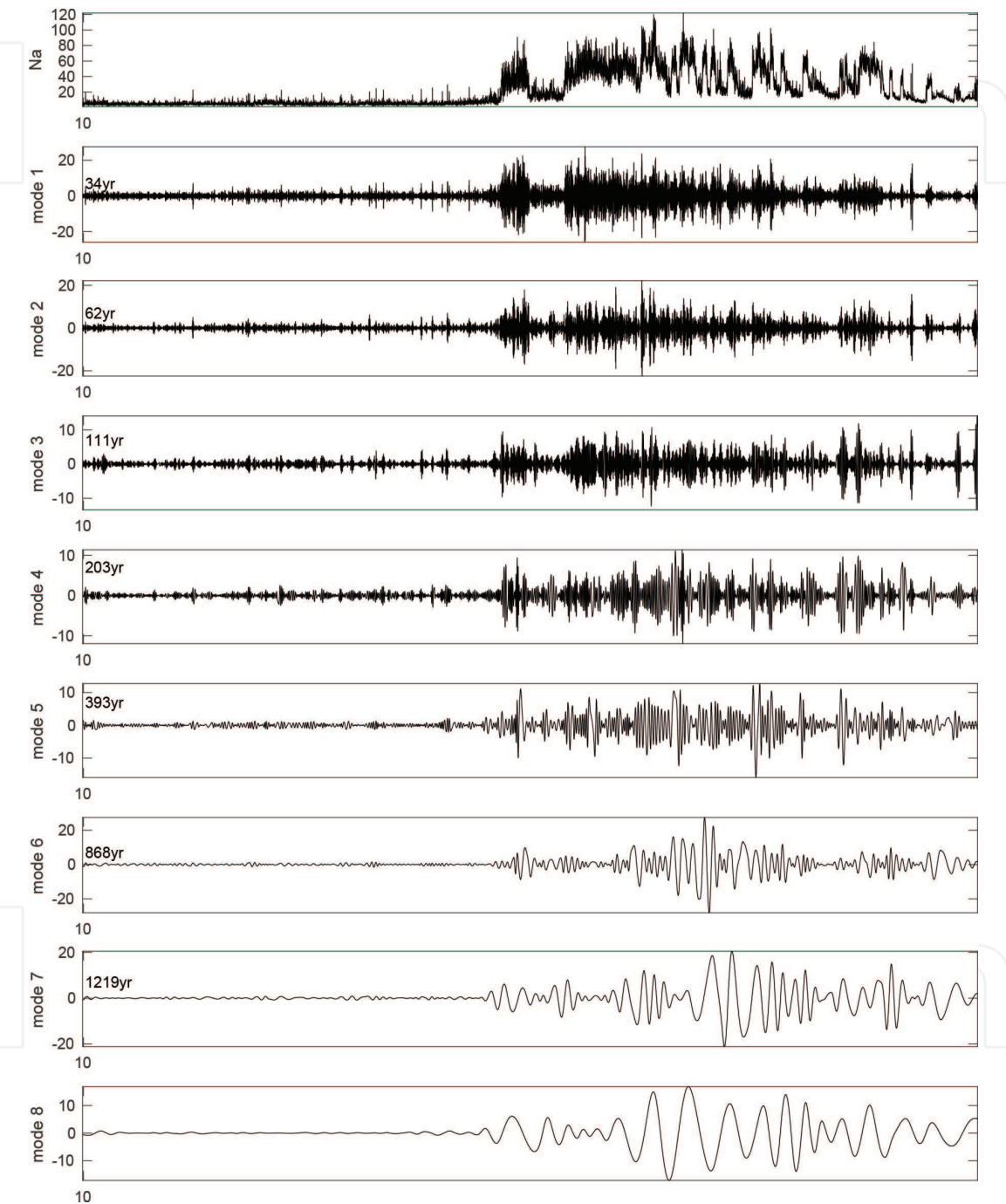
Figure 2. The GISP2 ice core data for the Na ion (upper panel). To obtain a uniformly sampled Na data set, we interpolated between the gaps in the original GISP2 unevenly spaced data and resampled with a time cadence of 10 years using the piecewise cubic Hermite interpolating polynomial, which preserves the shape of the data and respects monotonicity. This procedure works well for the most recent 50,000 years of the data set because there are no large unevenly spaced data gaps. The eight lower panels show the decomposition of the data variations into EMD modes. Each EMD mode varies in amplitude (seen in this figure) and frequency (can be estimated by the inverse quasi-period between zero crossings). The inverse frequencies of the EMD modes are shown in the left upper corner for each mode. At any given time, the sum of these modes equalizes the data. The mode amplitudes are scaled to the maximum of the data. The decrease in the amplitudes of variations at about 11,000 ybp is evident in all panels.
