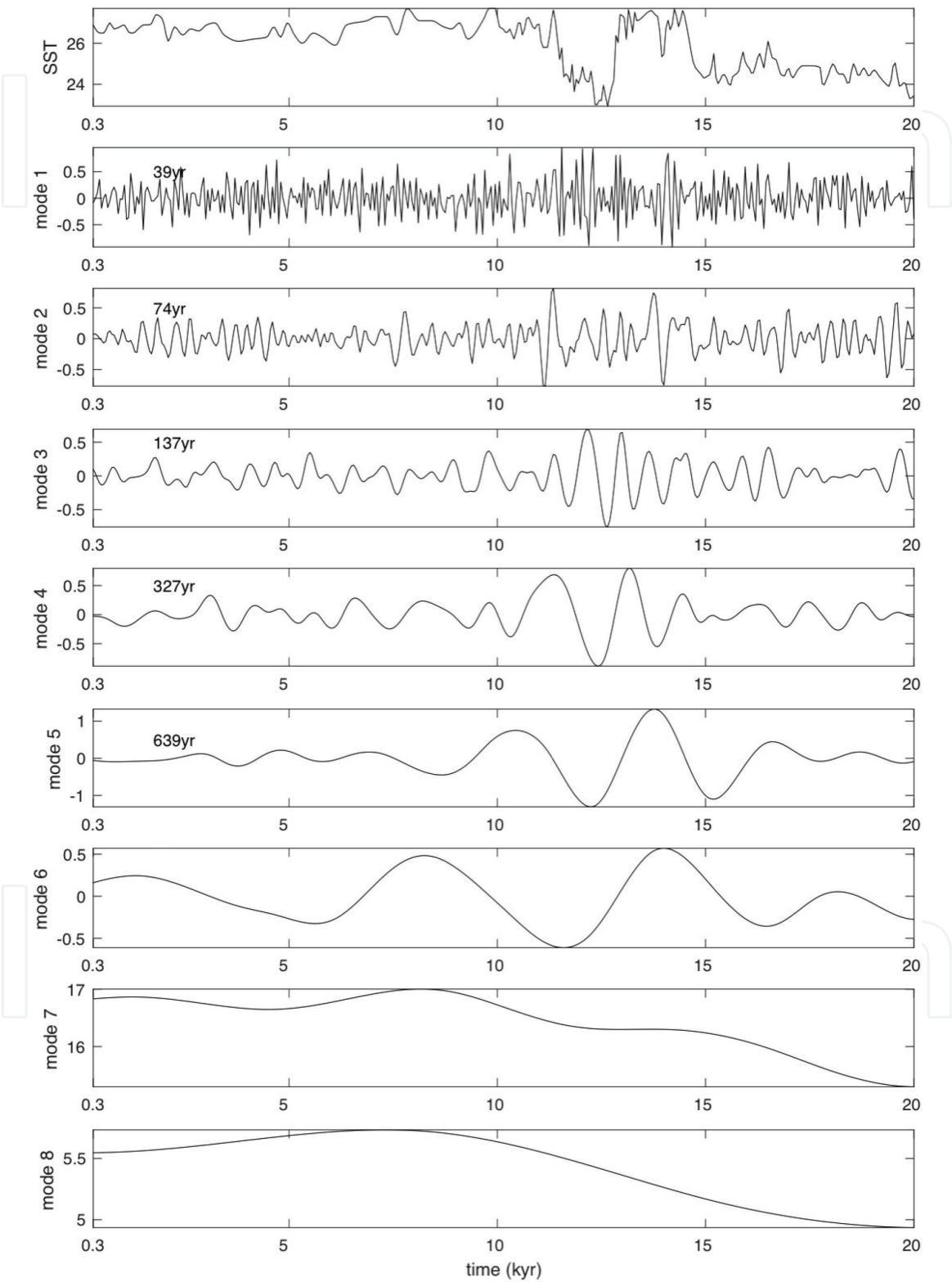
Figure 4. (Left rows) Top most panel shows the SST data in the Cariaco Basin, and the lower panels show the amplitudes of the EMD modes with the mean quasi-periods marked on the left side. Compared with GISP2 (see Figures 2 and 3 ), these data have lower resolution, and the time interval without major data gaps is more limited. We interpolated the data with a 50-year time cadence in the time interval from 300 ybp to 20,000 ybp. Note the presence of ~1500-year period in these data as well as in the GISP2 data. The amplitudes of all modes are large before and during the YD and decrease when the YD ends.
