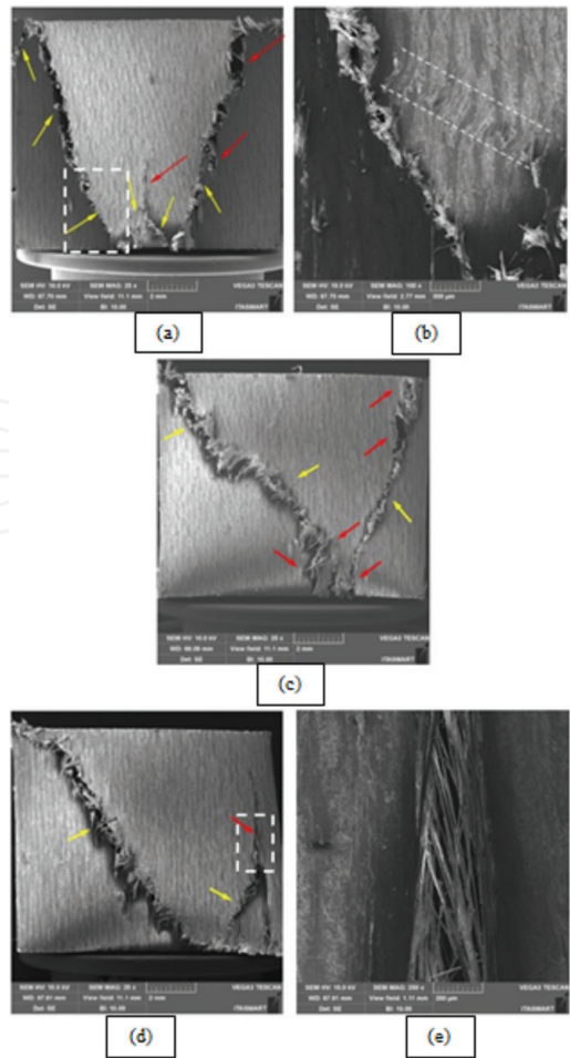
Figure 16. SEM images for PPSGFC tested under quasi-static strain rates. (a) 0.001\text{ s}^{-1} at 25\times , (b) marked zone in (a) at 100\times , (c) 0.01\text{ s}^{-1} at 25\times , (d) 0.1\text{ s}^{-1} at 25\times and (e) marked zone in (d) at 250\times .
