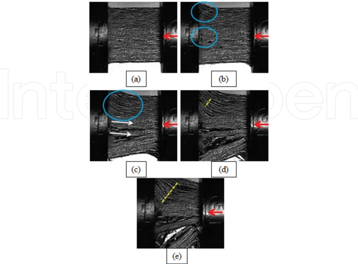
Figure 12. Images sequence taken by HSIS for PPSCFC tested at 832.2 s -1 .
