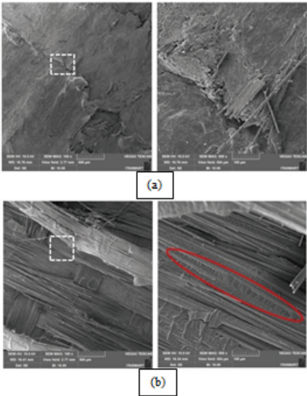
Figure 22. SEM images for PPSGFC tested at 891.1\text{ s}^{-1} . (a) “Melted” surface at 100× with 500× zoom of the marked zone, (b) “un-melted” surface at 100× with 500× zoom of the marked zone.
