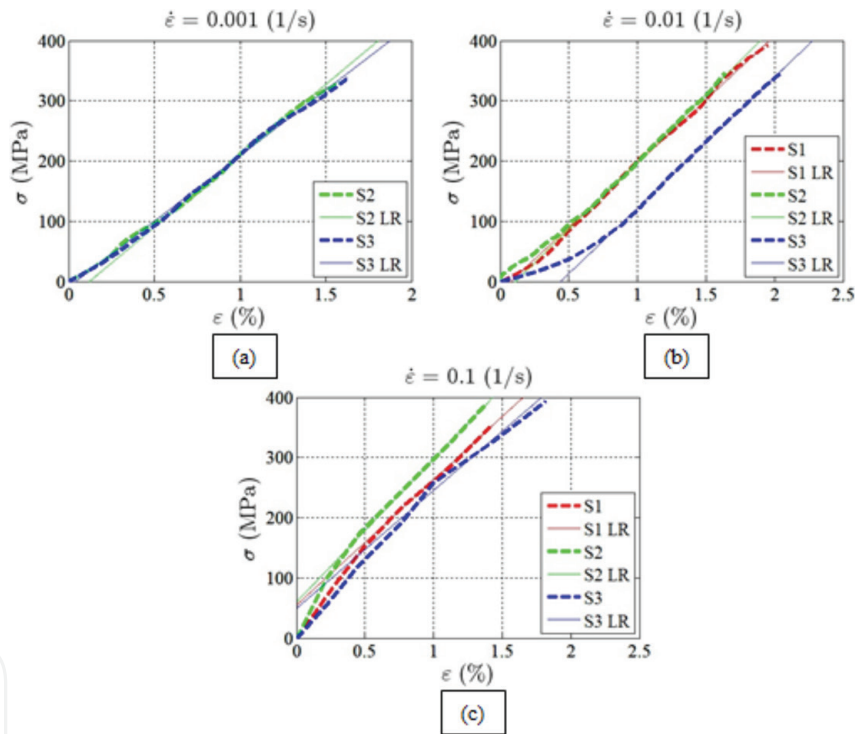
Figure 15. Stress-strain curve obtained for PPSCFC under compression at (a) 0.001 s -1 , (b) 0.01 s -1 and (c) 0.1 s -1 .
