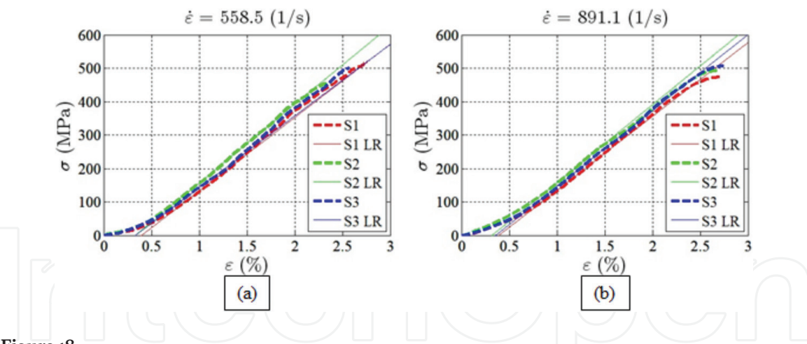
Figure 18. Stress-strain curves obtained under dynamic regime for PPSGFC: (a) 558.5\text{ s}^{-1} and (b) 891.1\text{ s}^{-1} .
