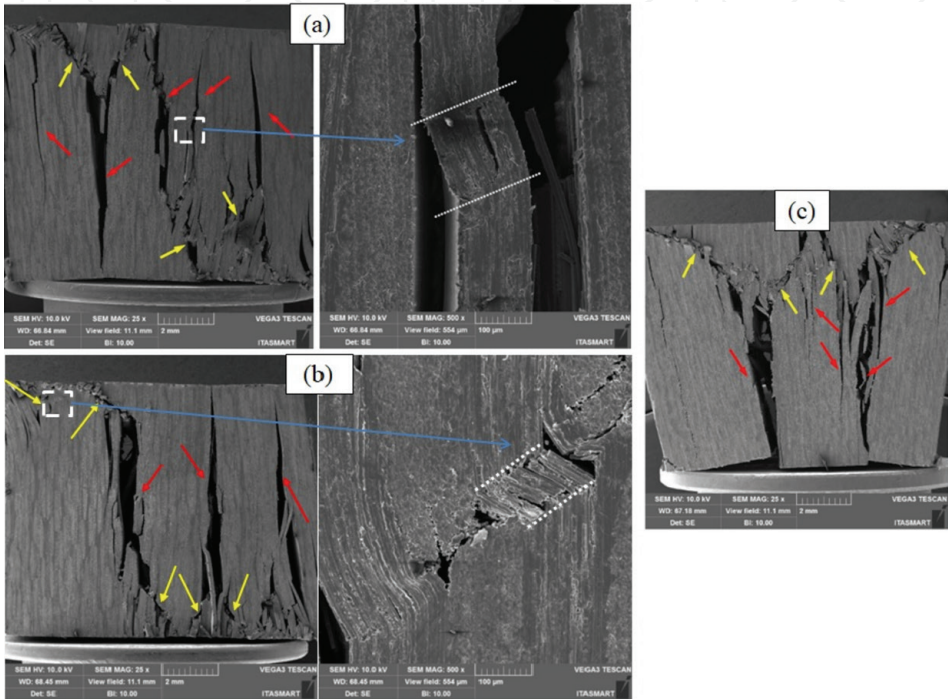
Figure 7. Quasi-static failure modes observation by SEM for PPSCFC under (a) 0.001\ s^{-1} (at 25 \times with amplified zone at 500 \times ), (b) 0.01\ s^{-1} (at 25 \times with amplified zone at 500 \times ) and (c) 0.1\ s^{-1} .
