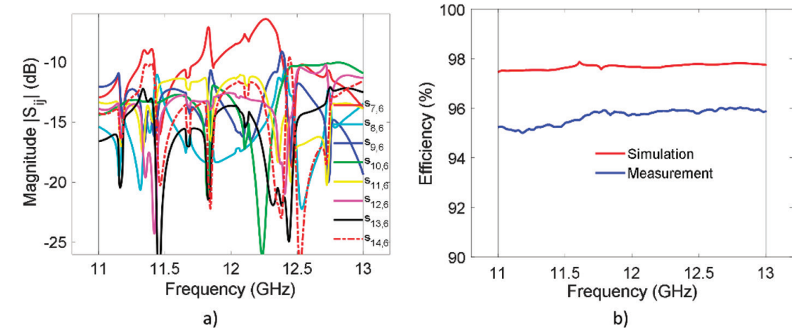
Figure 11. (a) Measured isolation response of the 16-way Ku-band power combiner: Transmission between the output port 6 (see the inset in Figure 9b) and the adjacent output ports of a middle of the combiner, i.e., the S_{7,6} S_{8,6} etc. until S_{14,6} parameter. (b) Comparison between the simulated and measured combining efficiency.
