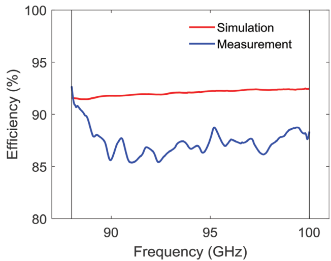
Figure 15. Comparison between the simulated and measured combining efficiency of the 5-way W-band power radial combiner.
