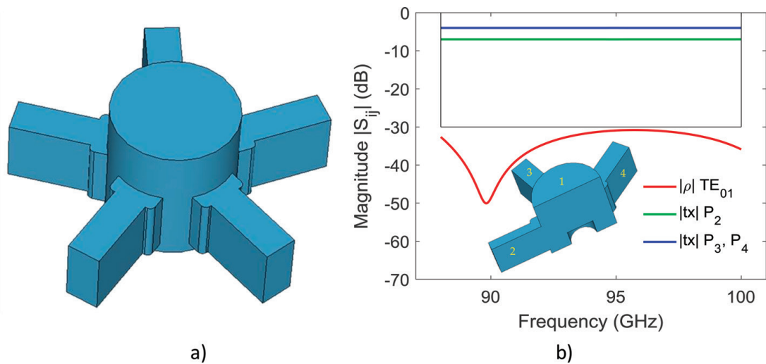
Figure 8. (a) 3D CAD view of the 5-way divider. (b) Simulated response of the reflection coefficient for the circular waveguide TE 01 cir mode, and the transmission to the TE 10 rec rectangular ports (from TE 01 cir ) (only half of the structure); in the inset, a 3D CAD view including the port numbering is shown.
