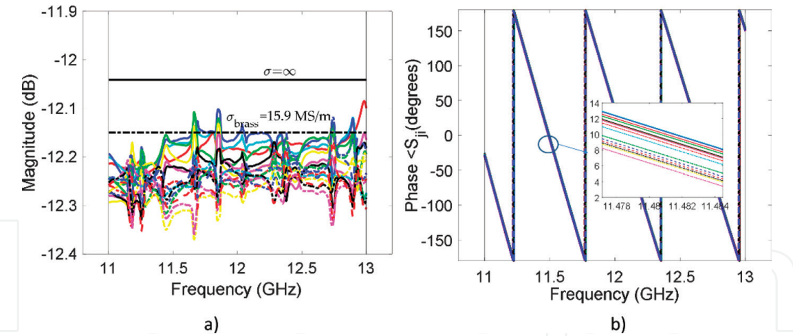
Figure 10. (a) Measured insertion loss of the 16-way Ku-band combiner compared with the theoretic value assuming perfect conductor ( \sigma = \infty , -12.04 \text{ dB} ), and the average value simulated corresponding to the brass conductivity ( \sigma_{\text{brass}} = 15.9 \text{ MS/m} , -12.15 \text{ dB} ). (b) Measured phases of the 16-way combiner from port 1 to ports 2–17, with a detail in the inset.
