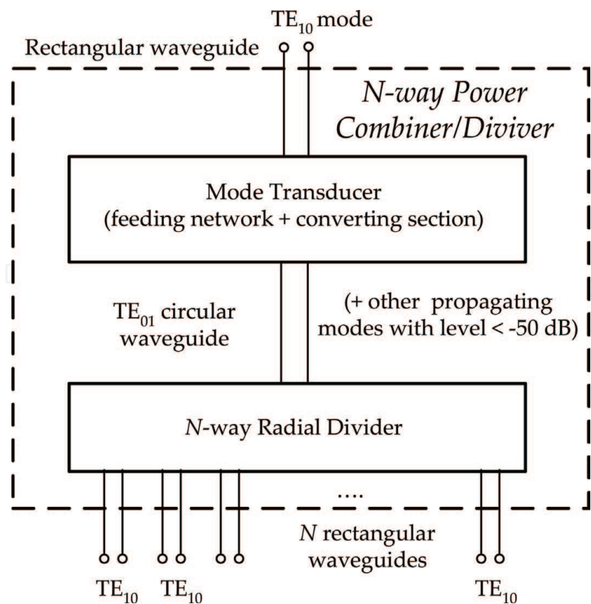
Figure 1. Scheme of the radial power combiner (or divider) made up of (i) the mode transducer between the rectangular waveguide TE_{10} mode and the circular waveguide TE_{01} mode, and (ii) the N -way radial divider (or combiner) dividing the power carried by the circular waveguide TE_{01} mode into N rectangular waveguide TE_{10} modes.
