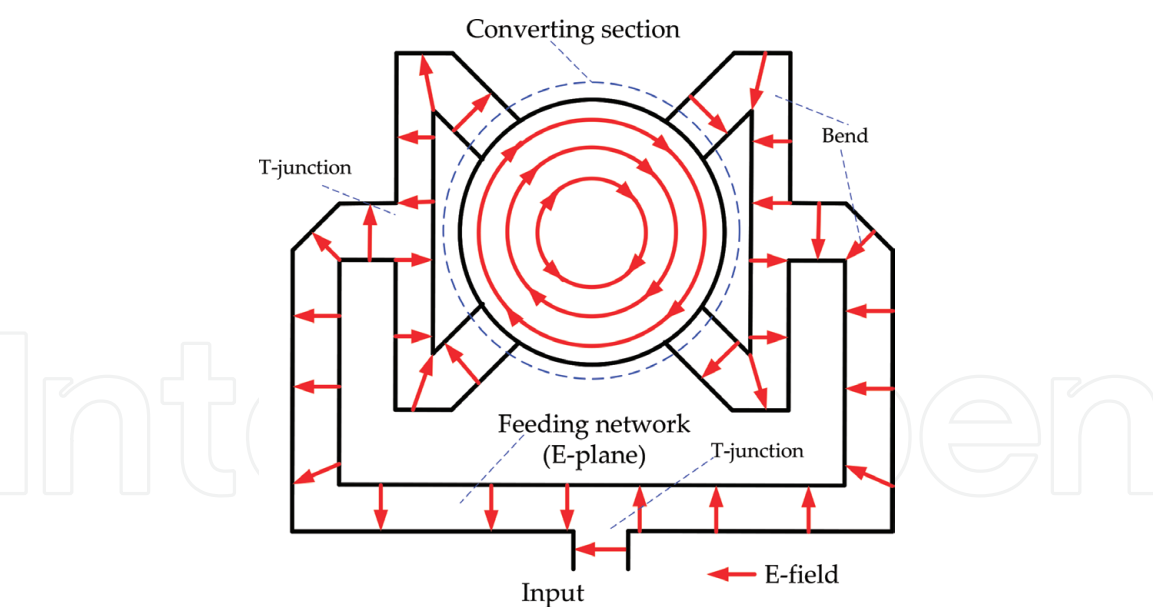
Figure 2. Scheme of a sidewall coupling for a circular waveguide TE_{01} mode transducer, showing the electric field lines, the converting-section (dashed circle) excited in its four sides, and the input feeding network (with E-plane T-junctions and waveguide bends).
