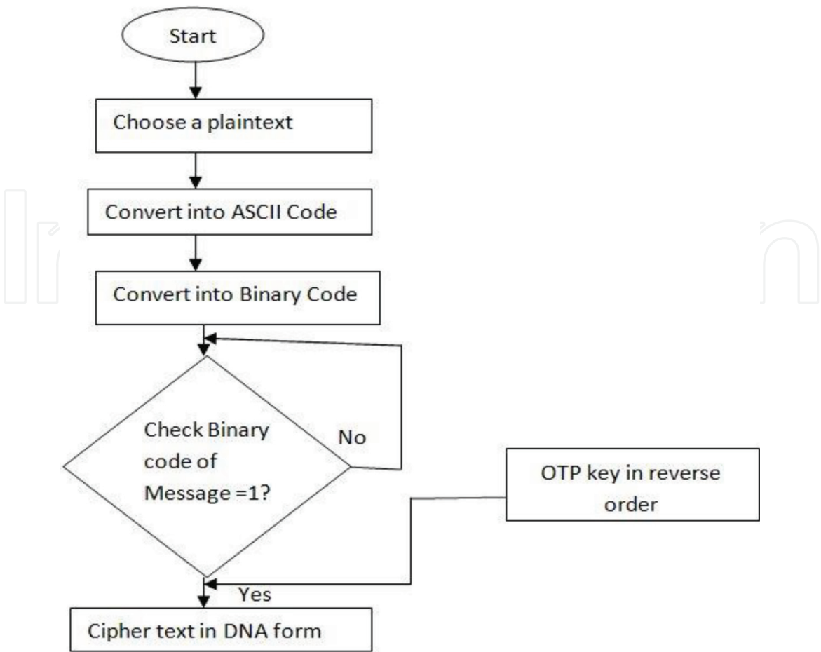
Figure 1. Flow chart of DNA hybridization encryption.
