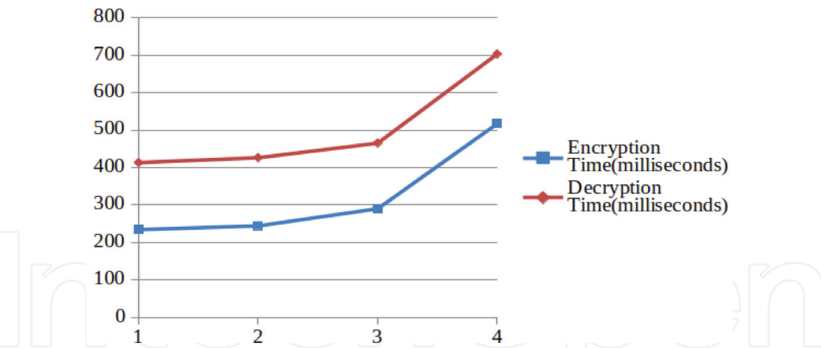
Figure 3. Analysis of encryption and decryption times of DDHO algorithm.
