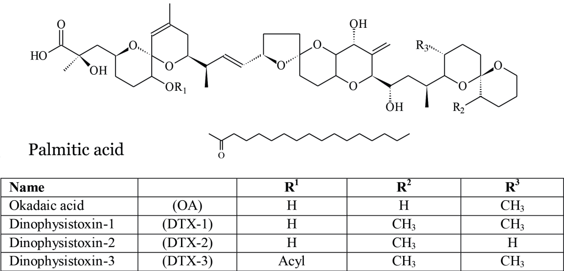
Figure 2. Chemical structures of okadaic acid group and analogues [33, 34].
