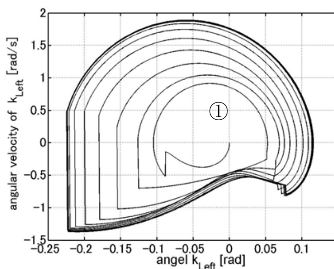
Fig. 8. Phase Plane Locus in Sagittal Plane
