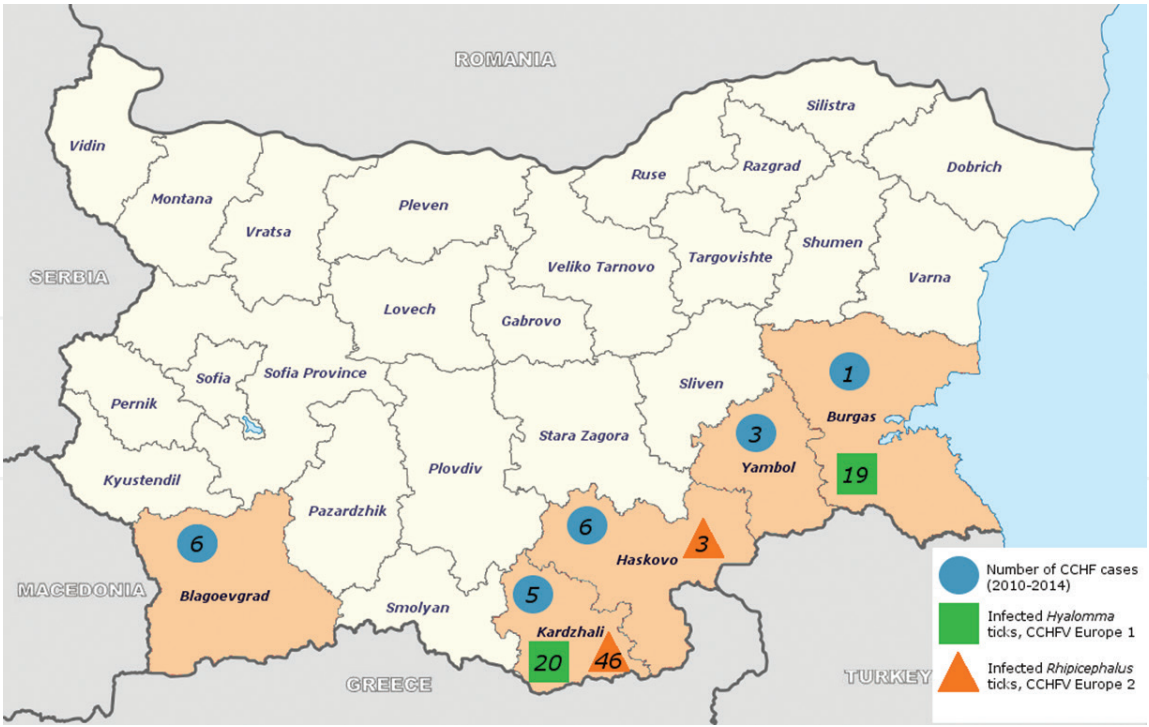
Figure 2. Detection of CCHF virus lineages Europe 1 and Europe 2 in tick from Bulgaria.
