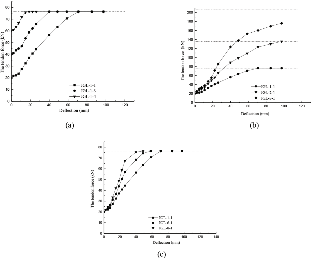
Figure 5. Cable internal force deflection curve. (a) The initial tendon force, (b) sectional area of cable, and (c) sag of cable. *The horizontal dotted line represents the tensile force at which the external prestressing tendon begins to fracture.
