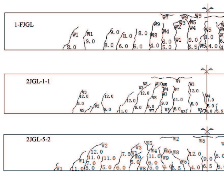
Figure 13. Beam crack mapping. 1-FJGL, 2JGL-1-1, 2JGL-5-2.
