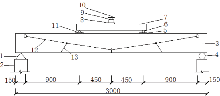
Figure9. Schematic diagram for loading setup (the unit used in the figure is mm). Notes: (1) fixed hinged support; (2) buttress; (3) test beams; (4) rolling hinged support; (5) backing plate; (6) rolling hinged support; (7) distributive girder; (8) jack; (9) pressure sensor; (10) reaction beam; (11) rolling hinged support; (12) wire rope; and (13) web member.
