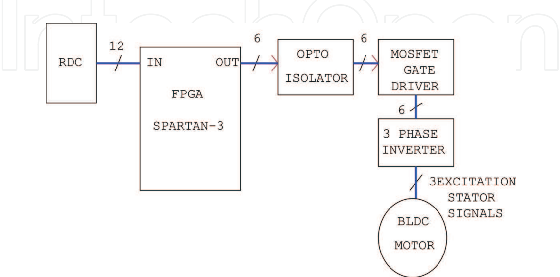
Figure 3. FPGA as open loop BLDC motor controller.
