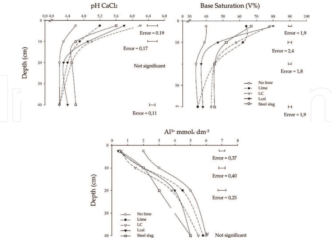
Figure 1. pH, base saturation (V%), and Al 3+ content at different depths of a dystrophic Red Latosol at 27 months after surface application of lime, centrifuged sewage sludge (LC), steel slag, and lama cal (Lcal) in the no-tillage system (source: [22]).
