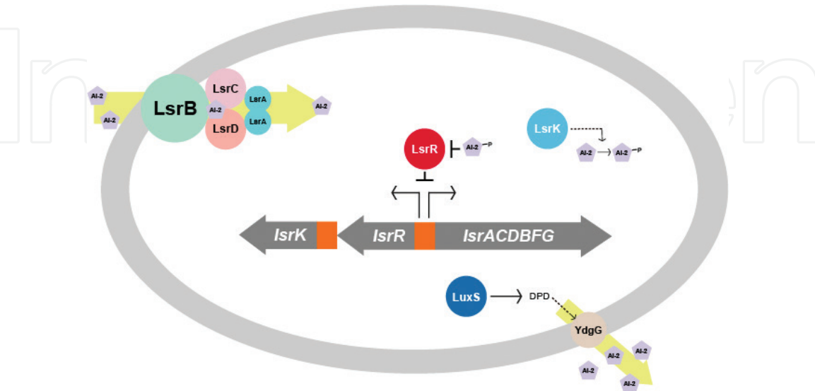
Figure 2. Regulatory mechanisms of the lsr /AI-2 circuit in E. coli . AI-2 is imported by the Lsr transporter (LsrACDB) and in turn, is processed by LsrK, transforming to its phosphorylated form (AI-2P). As AI-2P binds LsrR, it relieves the repression of LsrR on the Lsr genes and accelerates AI-2 intake. LuxS produces DPD, the precursor of AI-2. The autoinducer is then transported out of the bacteria by YdgG (TqsA), a putative transporter belonging to the exporter superfamily [40].
