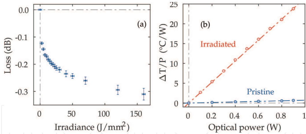
Figure 9. (a) Direct measurement of the loss as the PS980 fiber is irradiated. (b) Heating of the PS980 fiber as a function of the illumination power.
