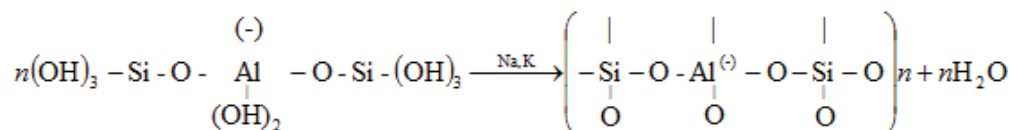
Figure 1. Formation of geopolymers: (A) poly(sialate) and (B) poly(sialate-siloxo).
