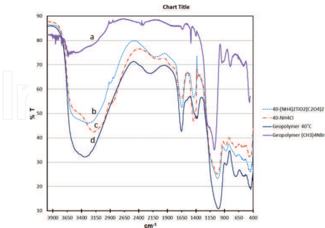
Figure 6. FT-IR of (a) geopolymer at 40^\circ\text{C} ion exchanged with (\text{CH}_3)_4\text{NBr} , (b) geopolymer at 40^\circ\text{C} ion exchanged with (\text{NH}_4)_2\text{TiO}_2(\text{C}_2\text{O}_4)_2 , (c) geopolymer at 40^\circ\text{C} ion exchanged with \text{NH}_4\text{Cl} and (d) geopolymer at 40^\circ\text{C} .
