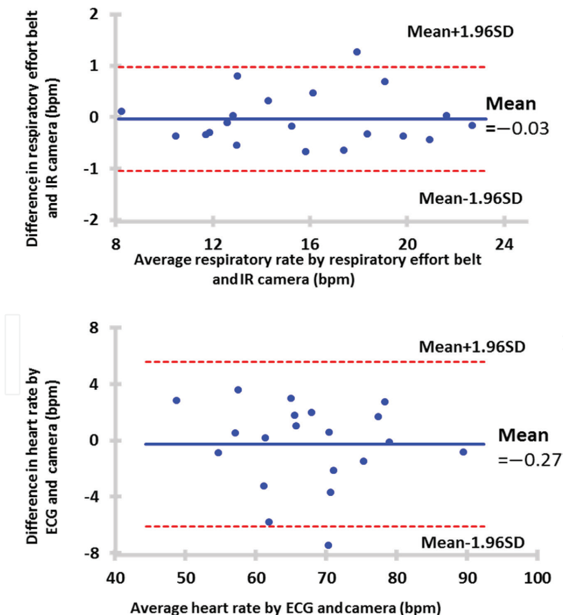
Figure 4. Plot of respiration/heart rate from Bland-Altman analysis.
