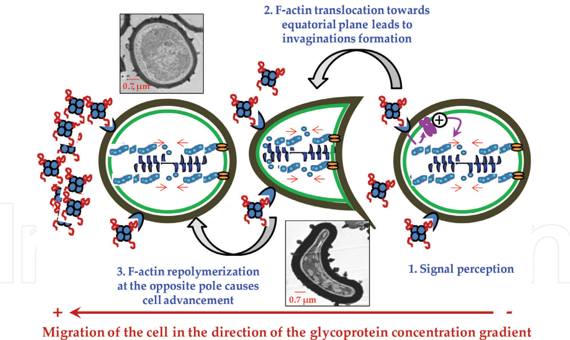
Figure 7. Scheme of movement of S. scitamineum cells during sugarcane-pathogen interaction that explain how motility of teliospores is due to contraction-relaxation episodes of the cytoskeleton. (1) chemoattractant glycoprotein released by sugarcane plants binds to specific receptors in fungal cell walls. As a result, the transduction signal that implies cytoskeleton reorganization is activated. (2) Polar cell invaginations are produced by interaction of myosin II with F-actin cytoskeleton. The translation of the actin filaments into the interior of the cell must begin at its less end, located in the equatorial plane of teliospore. This permits an increase of the cell volume in the front of advance and the retraction of the opposite pole, which produces cell invagination. (3) Repolymerization of F-actin in the front of cell produces the cell advancement. Representing: the glycoproteins; the receptor in fungal cell; the signal transducing proteins; the actin monomers; the F-actin; the myosin; the anchorage proteins; the cell wall; the plasmatic membrane; and the direction of retrograde flow. F-actin specific labeled ferritin can be seen in micrographs obtained by transmission electron microscopy (TEM).
