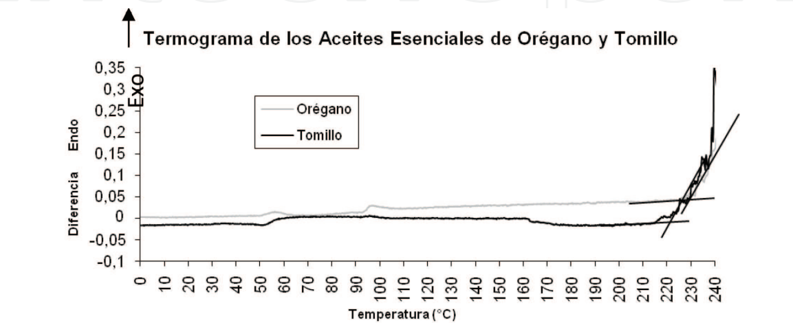
Figure 4. Thermogram of thyme and oregano essential oils.
