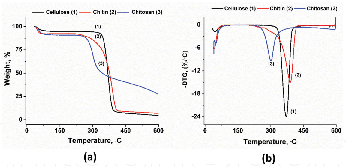
Figure 5. (a) TG and (b) DTG profiles of cellulose, chitin and chitosan.
