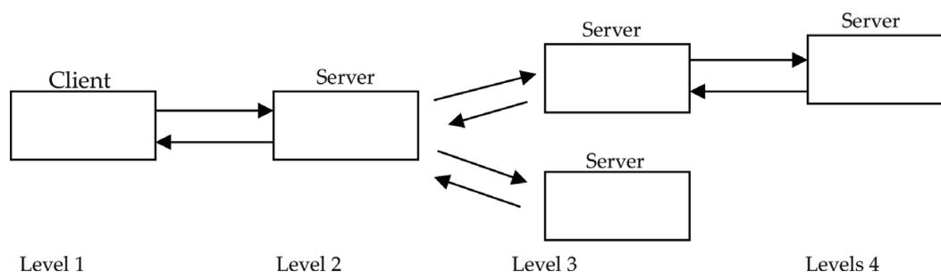
Figure 5. N-tier architecture.
