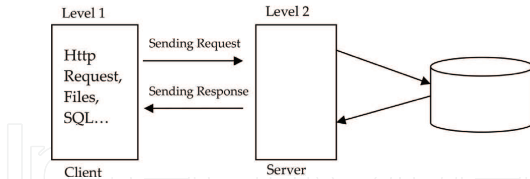
Figure 3. Two-tier architecture.
