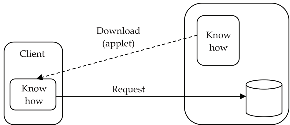
Figure 10. Code-on-demand.
