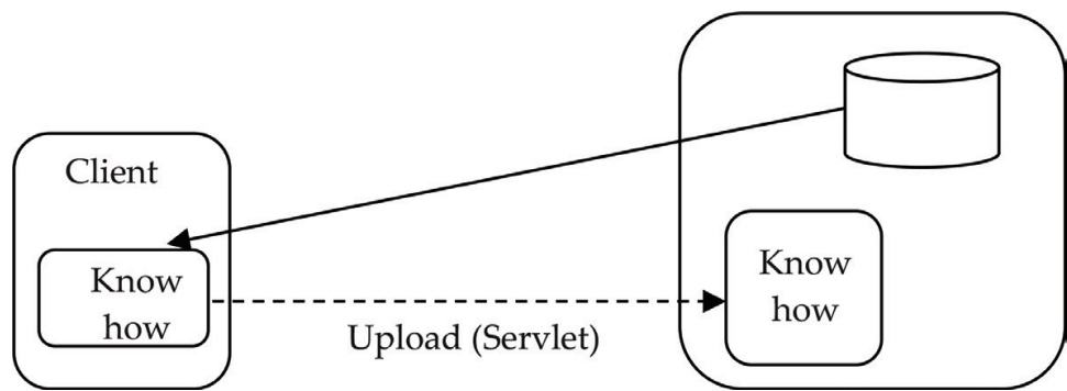
Figure 13. Remote evaluation.
