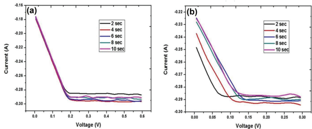
Figure 7. Potentiometric graphs of (a) duplex stainless steel and (b) ferritic stainless steel, respectively, at 0.5 M \text{H}_2\text{SO}_4 solution [30].
