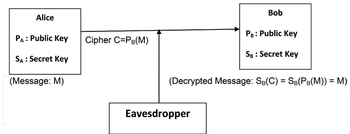
Figure 2. Public-key cryptosystem.
