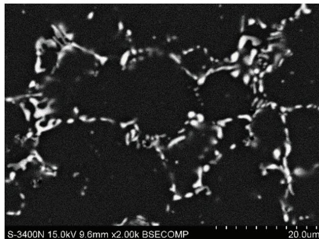
Figure 16. Coagulation of (\text{Al}, \text{Mg})_4\text{Sr} phase precipitates in die-cast AJ62 alloy after annealing for 4000 h at 350°C, SEM.
