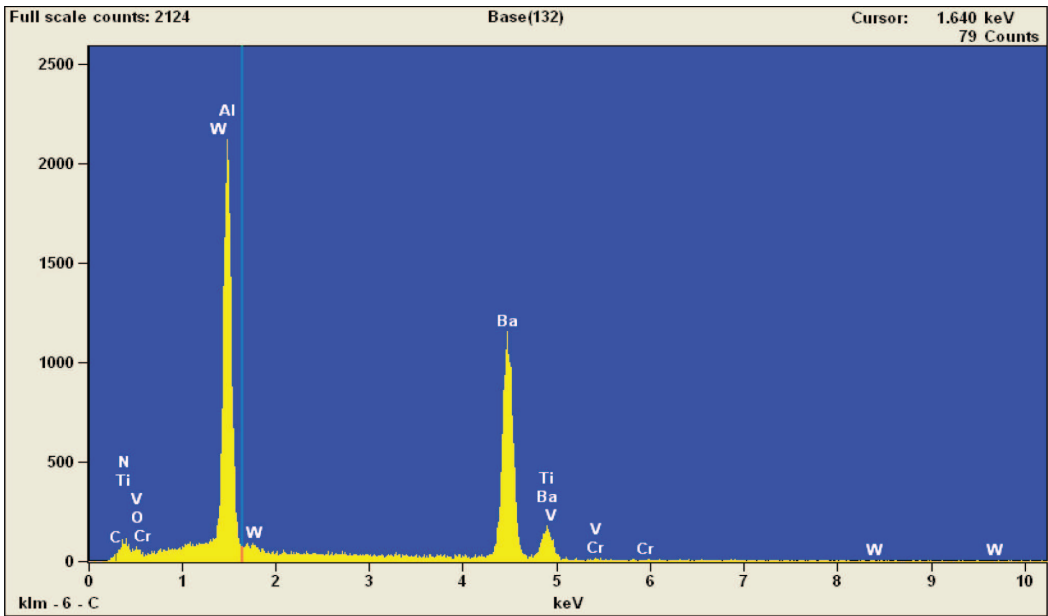
Figure 6. EDS spectrogram.
