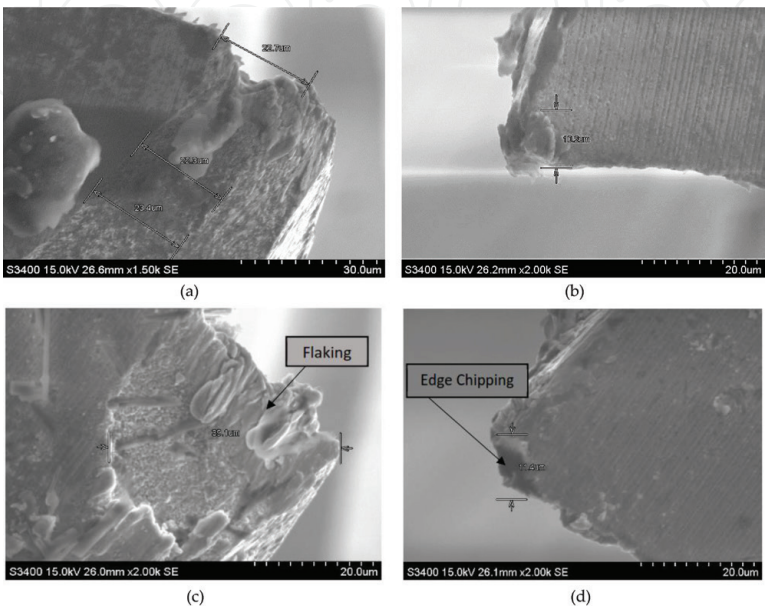
Figure 7. (a–d) Tool wear observation for uncoated tools.
