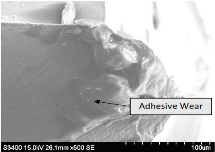
Figure 12. Coated AlTiN tool wear at 110,000 rpm.
