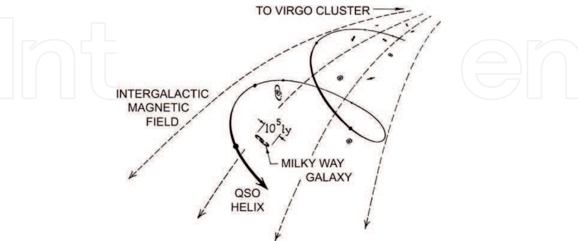
Figure 3. Helix of electrically charged QSOs within an intergalactic magnetic field originating in the Virgo Cluster of galaxies.
