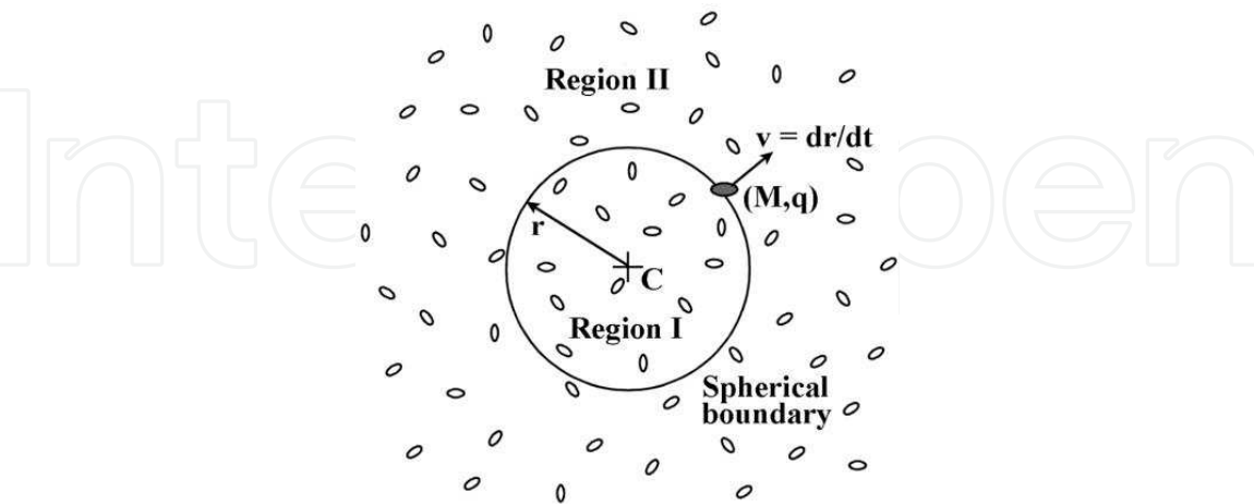
Figure 1. Division of universe into Region I and Region II to facilitate analysis. This figure has been previously published in: Ref. [3] ( http://www.physicsessays.org/browse-journal-2/product/1532-26-dietmar-e-rothe-the-case-for-a-gentler-bang-a-cosmology-of-gradual-creation.html ). It is reprinted with permission of Physics Essays Publication.
