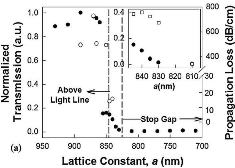
Figure 5. Lattice constant dependent transmission and propagating loss [45].
