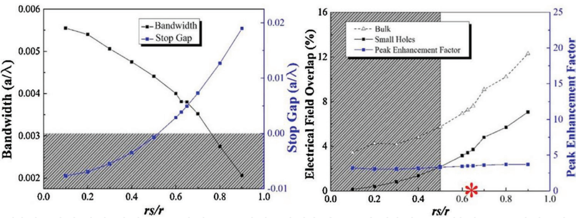
Figure 4. Optimization of rs/r according to bandwidth, stop gap electrical field overlap, peak enhancement factor [45].
