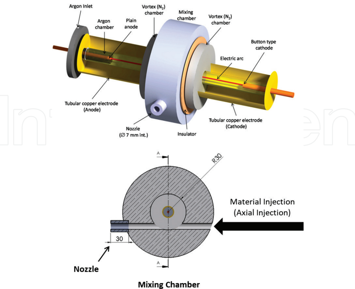
Figure 3. High velocity plasma spray with axial injection presented by Caliari et al. [21].
