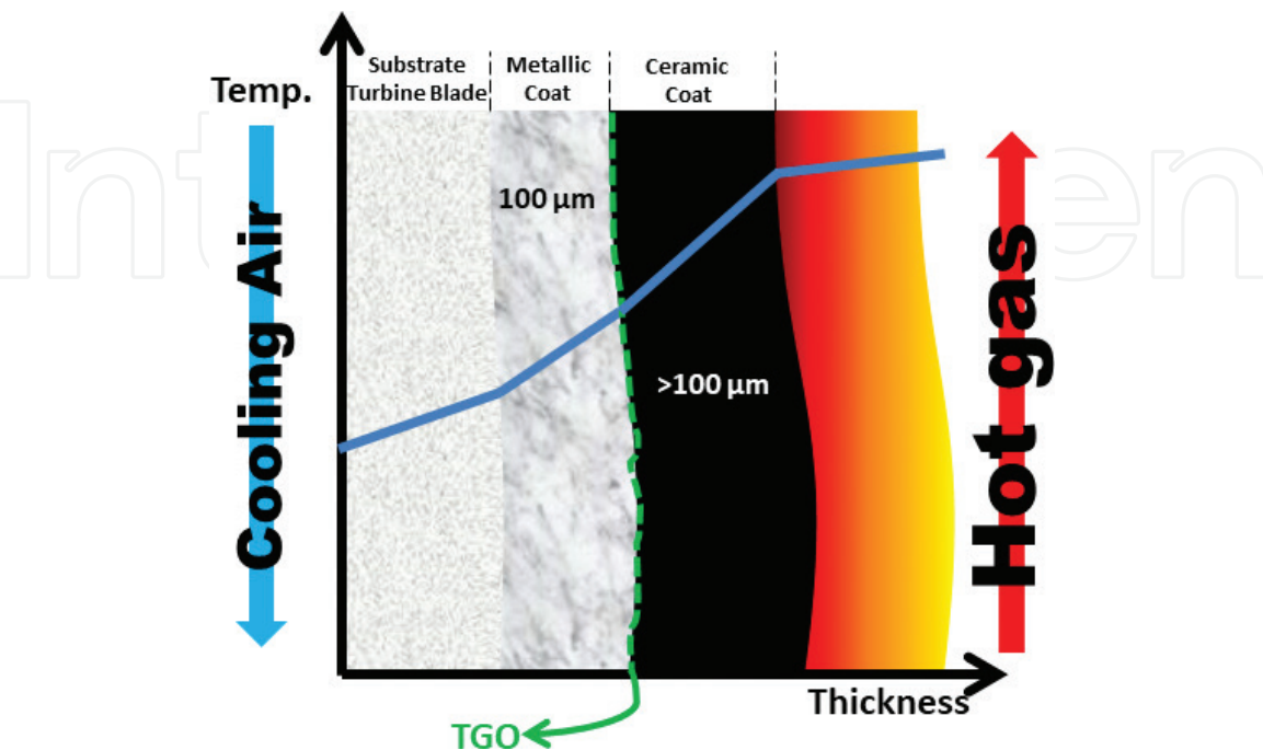
Figure 1. Thermal barrier coatings applied on turbine blade.
