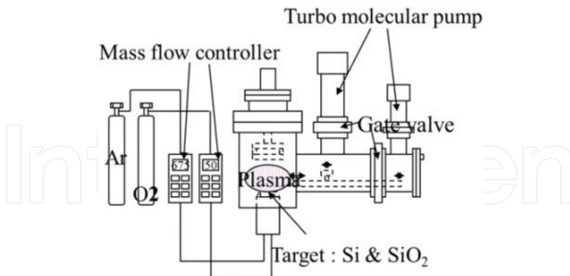
Figure 1. A schematic drawing of the ultrahigh vacuum radio frequency magnetron sputtering. Sputtering targets can be changed at each deposition program.
