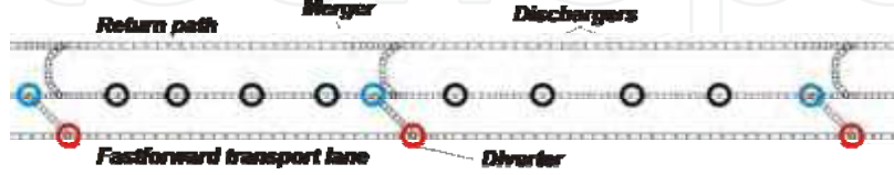
Figure 12. Area of the BHS layout with indication of diverters, mergers, and dischargers
