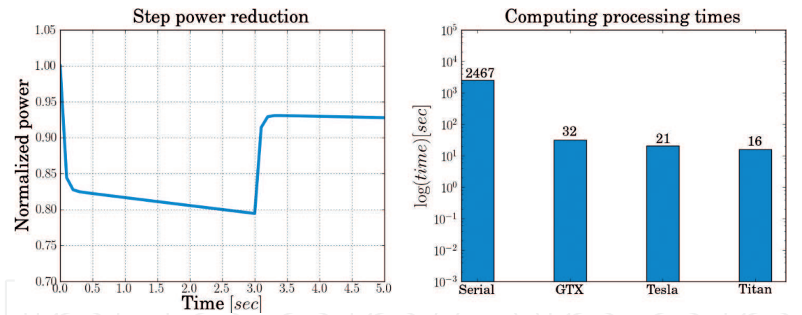
Figure 6. Simulation of a reactor power transient—serial and parallel processing.
