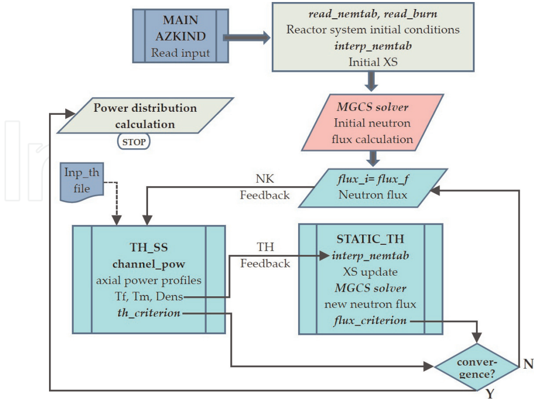
Figure 4. The NK-TH feedback process in AZKIND.
