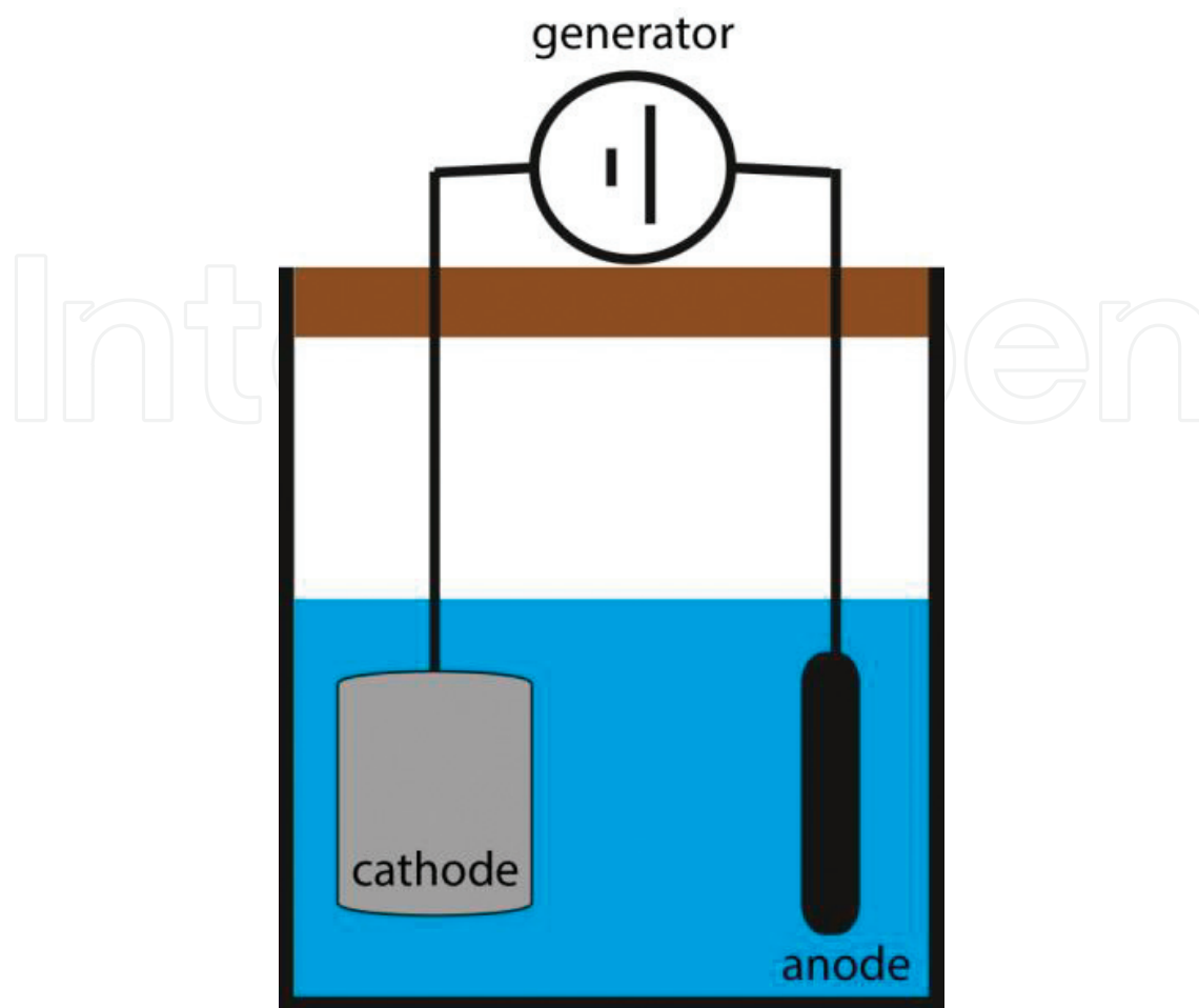
Figure 7. Simple deposition system of electrodeposition technique, the solution is an electrolyte that is deposited by electric current and moved from the anode to the cathode where the material is deposited; the variables are electrolyte concentration and amperage.
