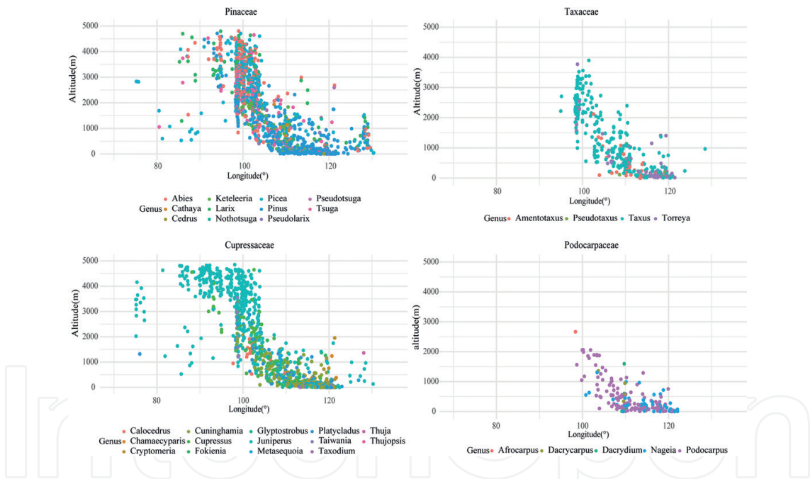
Figure 5. Altitudinal distribution of conifer families along longitude in China.
