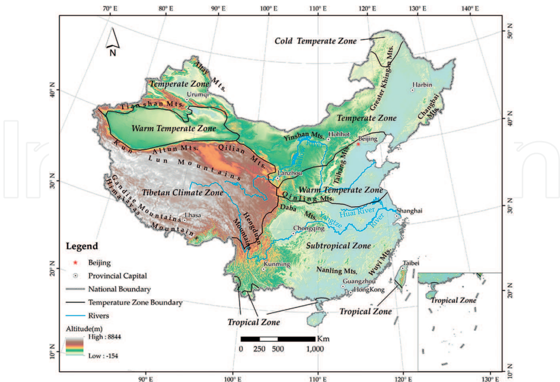
Figure 1. Distribution of the main mountain ranges in China.
