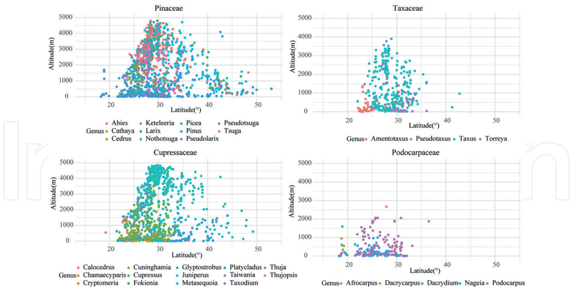
Figure 4. Altitudinal distribution of conifer families along latitude in China.
