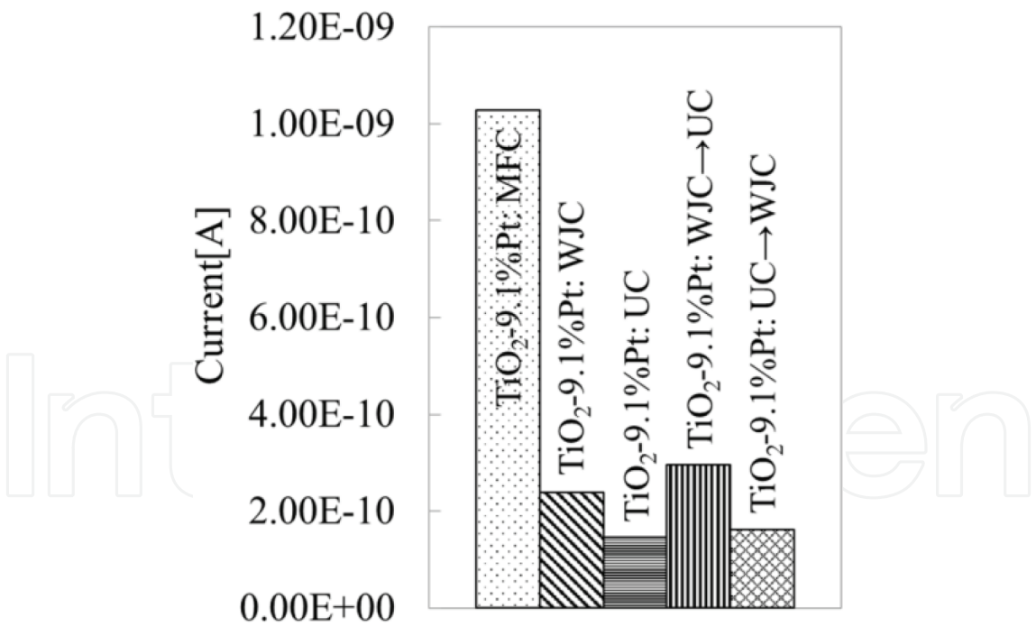
Figure 21. Oxygen generation from various cavitation processed TiO 2 particles supported by Pt particles.
