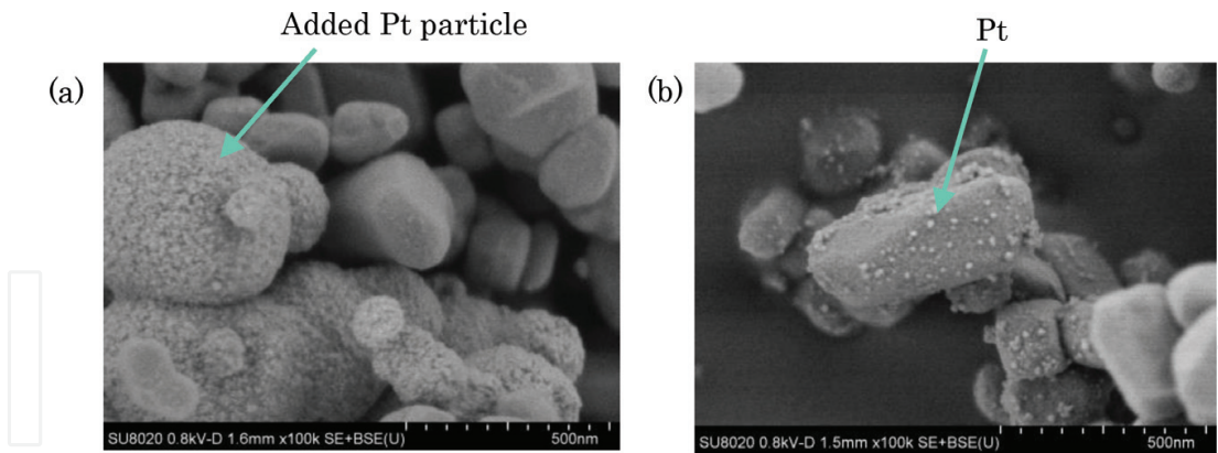
Figure 15. FE-SEM images of \text{TiO}_2 particles supported by Pt particles as a co-catalyst after cavitation processing ( \times 100,000 ). (a) Pt particle mixed with \text{TiO}_2 and (b) minute Pt particles supporting \text{TiO}_2 particles.
