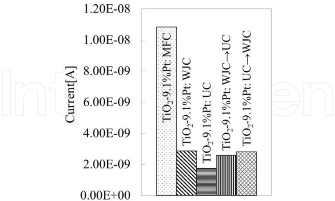
Figure 20. Hydrogen generation from various cavitation processed TiO 2 particles supported by Pt particles.
