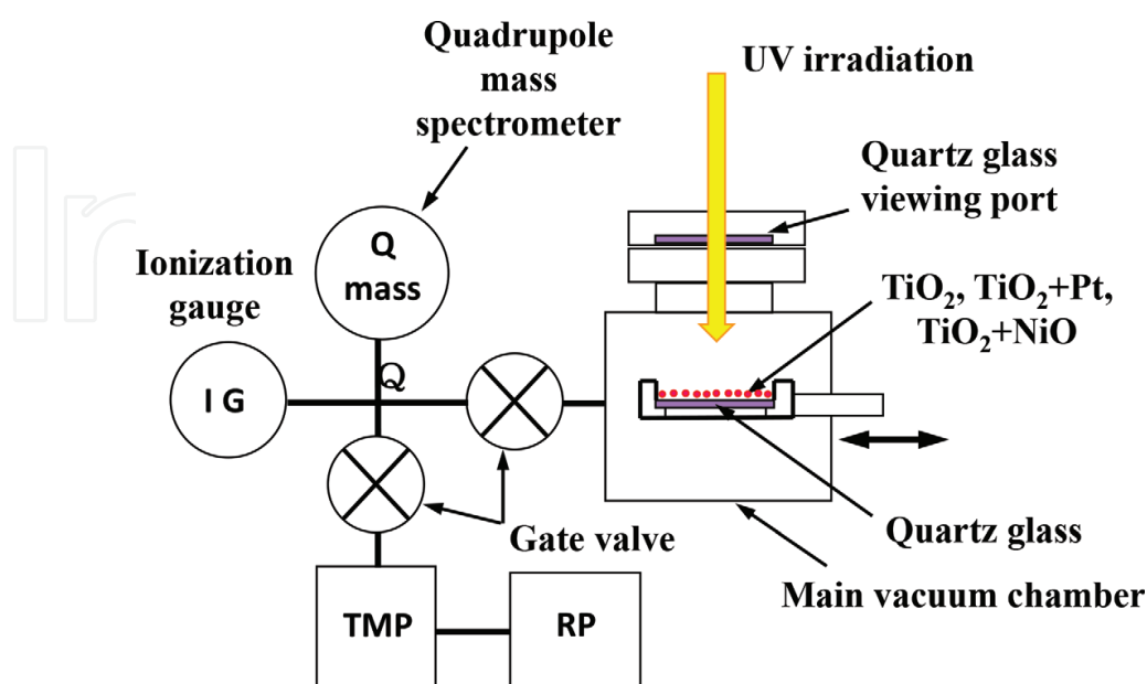
Figure 12. Schematic of equipment used in the present photocatalytic experiments.
