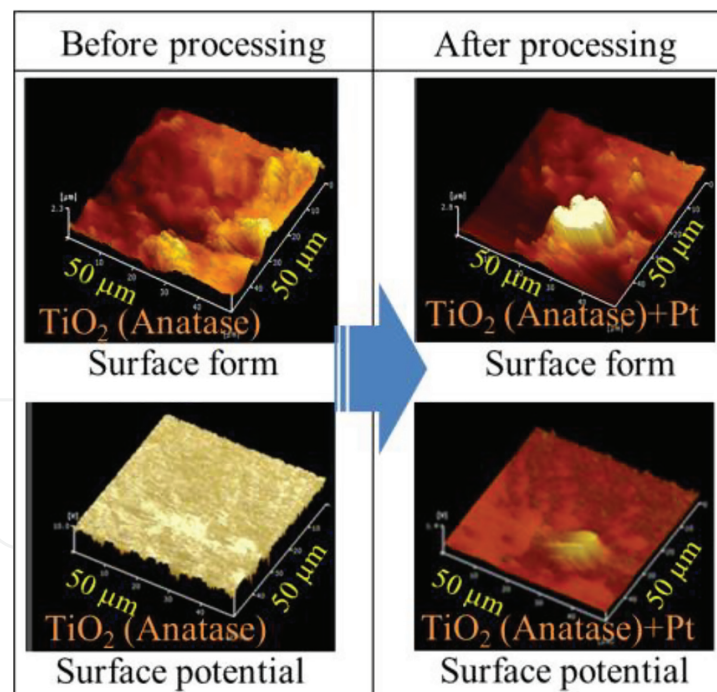
Figure 23. Results of surface potential imaging (Anatase-type TiO 2 ).
