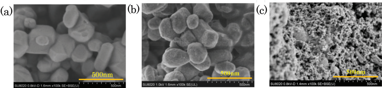
Figure 16. FE-SEM images of titanium oxide particles (a) as-received, (b) after WJ processing, (c) after MFC processing ( \times 100,000 ).
