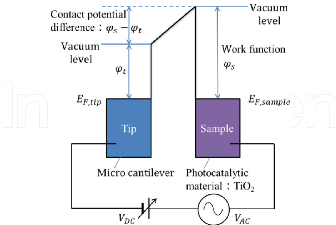
Figure 13. Schematic diagram of the Kelvin force microscope.
