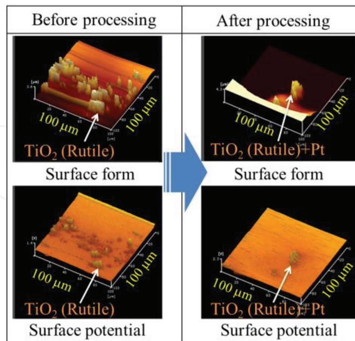
Figure 22. Results of surface potential imaging (Rutile-type TiO 2 ).
