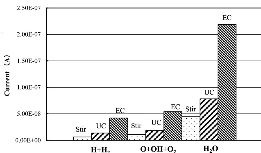
Figure 17. Comparison of EC processing, UC processing and stir processing with regard to amount of gas generation from \text{TiO}_2 particles supporting Pt ( \text{TiO}_2 + 9.1 \text{ wt\% Pt} ) under UV irradiation.
