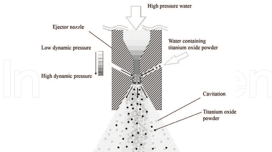
Figure 11. Cavitation processing of a photocatalyst powder by the ejector reactor.
