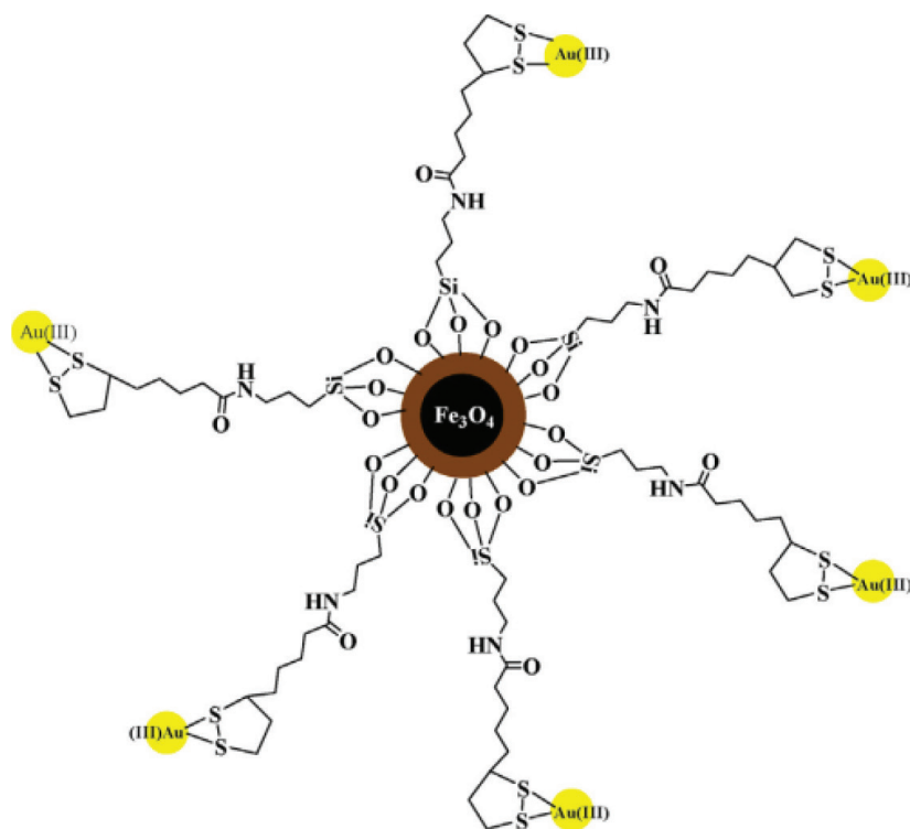
Figure 3. Possible interaction between \text{RS-SR-NH-SiO}_2@\text{Fe}_3\text{O}_4 and \text{Au(III)} ions [31].
