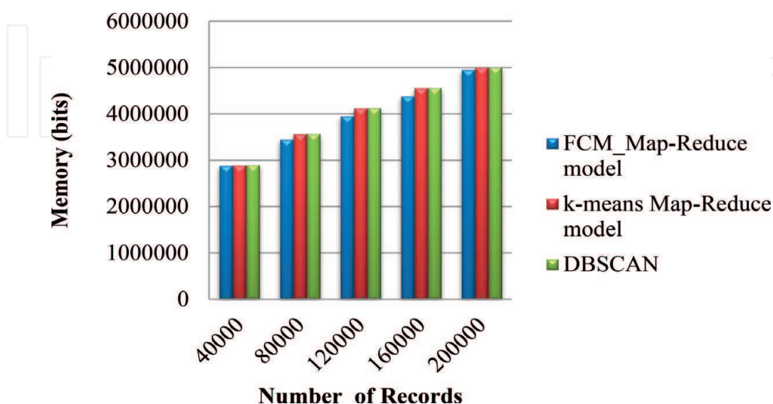
Figure 4. Memory requirement for FCM based Map-Reduce and k-means based Map-Reduce model.
