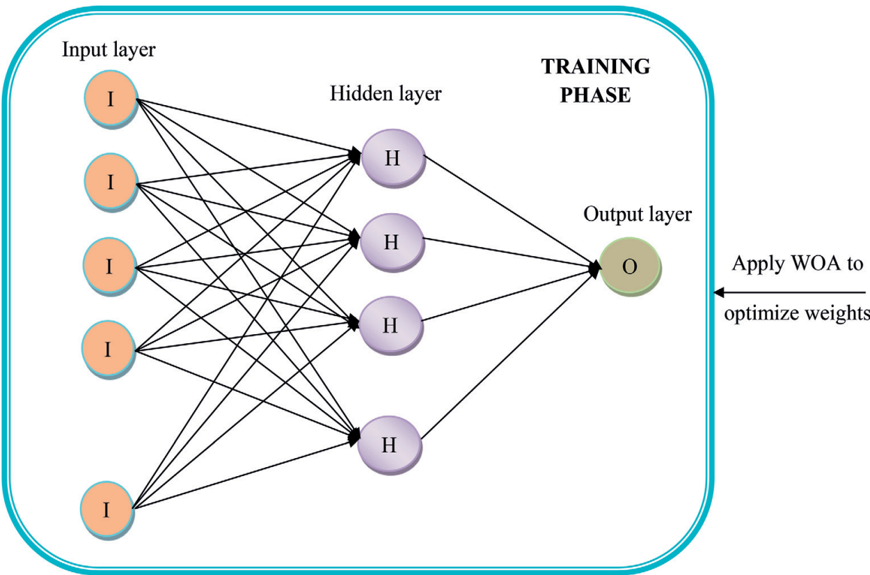
Figure 2. Proposed adaptive artificial neural network.
