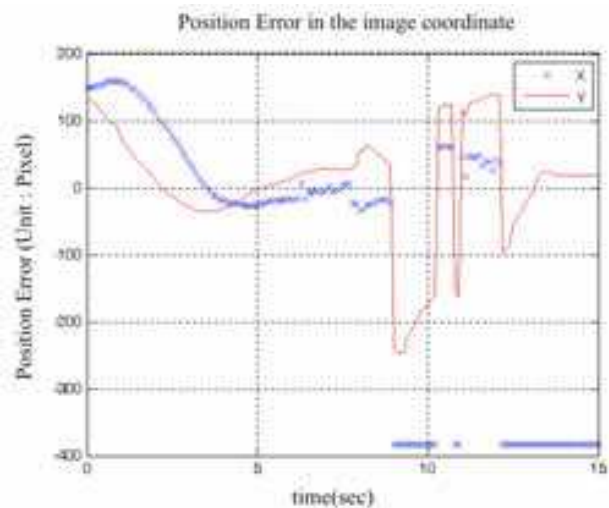
Fig. 24. Position error (unit: pixel) in the image coordinate. The vision-guidance control was applied through all intervals. (1) t = 0\text{-}9\text{seconds} : Errors are decreasing. In this interval, all 5 lights were in the viewing range of the camera. The AUV was able to estimate the center precisely. (2) t = 9\text{-}15\text{seconds} : one or more lights were out of the viewing range of the camera. Precise estimation of the center became impossible. The oscillation was caused by the defect of information from image processing rather than actual motion of the AUV.
