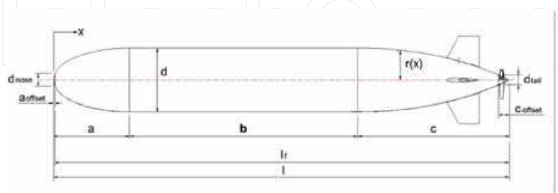
Fig. 3. Hull contour of ISiMI AUV.
