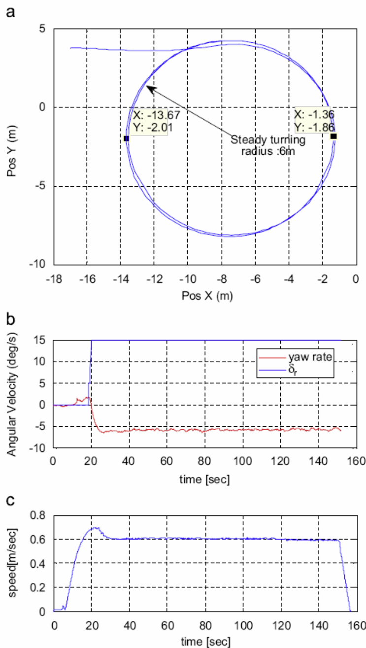
Fig. 13. Experimental results of open-loop turning test: (a) turning radius; (b) steady state turning rate and (c) steady state turning speed.
