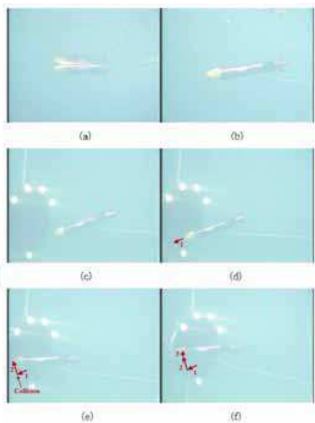
Fig. 25. Docking : Grabbed images by an underwater camera (Arrows indicate moving directions of the AUV): (a): ISiMI starts, (b): She cruises to (c) the dock, (d): An imprecise approach near the dock, (e): After a collision, she rebounded, and (f): She could not enter the dock.
