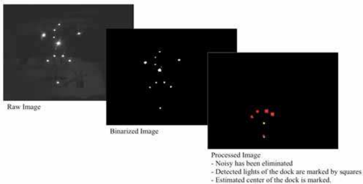
Fig. 19. Image process sequence (test screenshots was used): Raw image (left), binary image- some noisy luminaries remain. (center), and processed image - elimination of noisy luminaries and discrimination of the dock lights.
