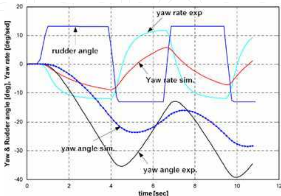
Fig. 12. Experimental results of open-loop zigzag test.
