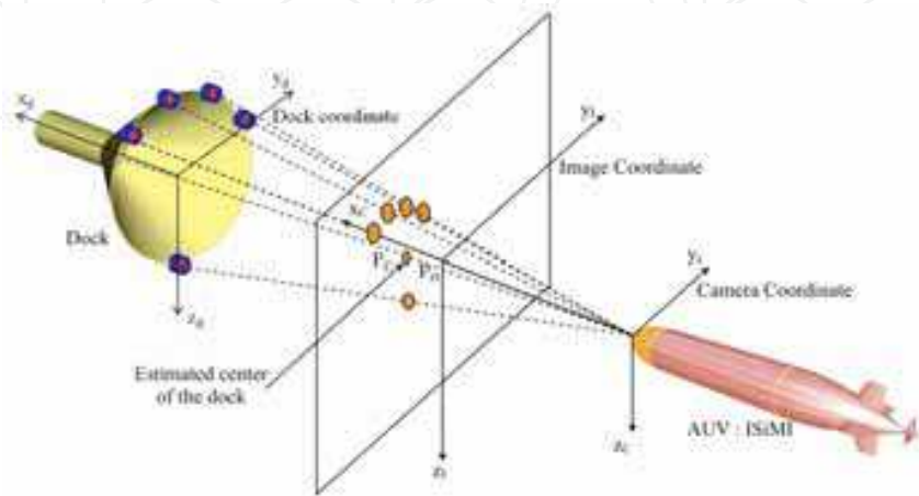
Fig. 17. Coordinates of the vision system.
