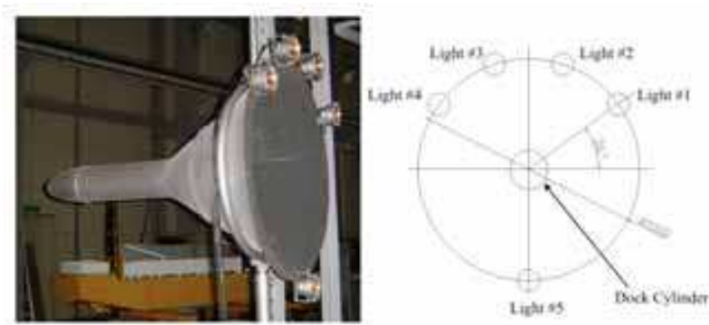
Fig. 16. The docking device with five lights around the rim of the entrance: The location and intensity of the lights is adjustable. (Left) Photo of the dock configuration and (Right) arrangement of the lights.
