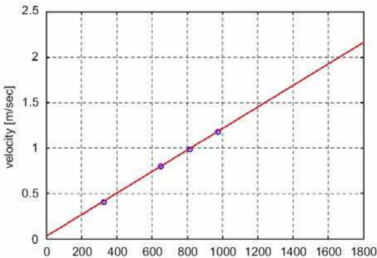
Fig. 11. Advanced speed test of ISiMI.
