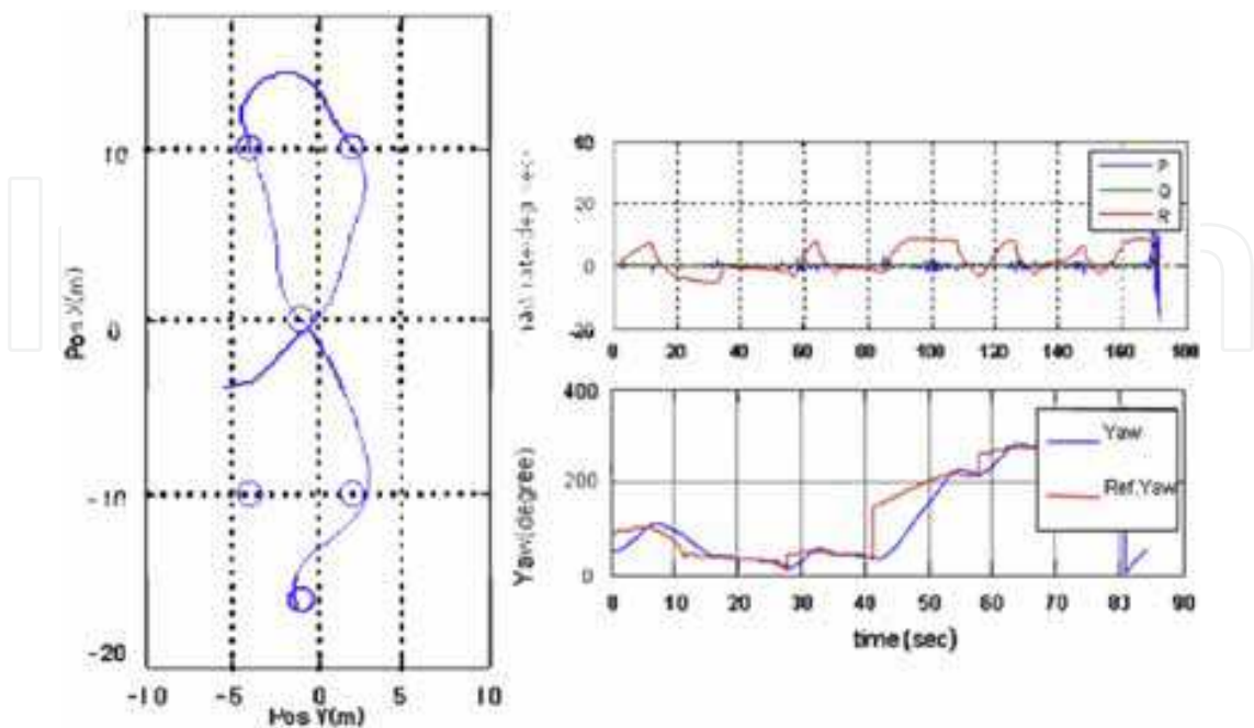
Fig. 15. Experimental results of waypoint tracking.
