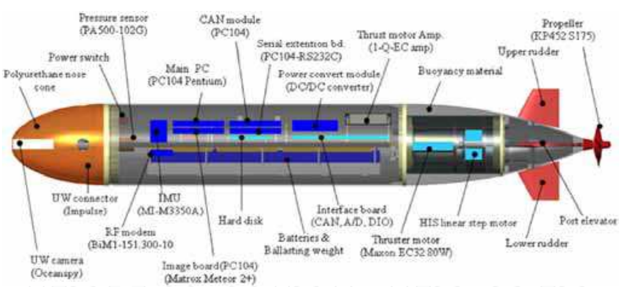
Fig. 6. General arrangement of the AUV ISiMI system.
