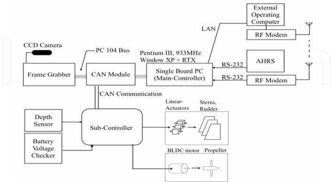
Fig. 4. Control system diagram of ISiMI.
