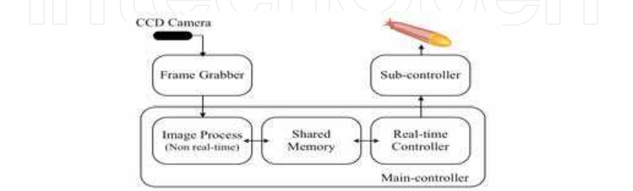
Fig. 7. Block diagram of the vision-guidance system.
