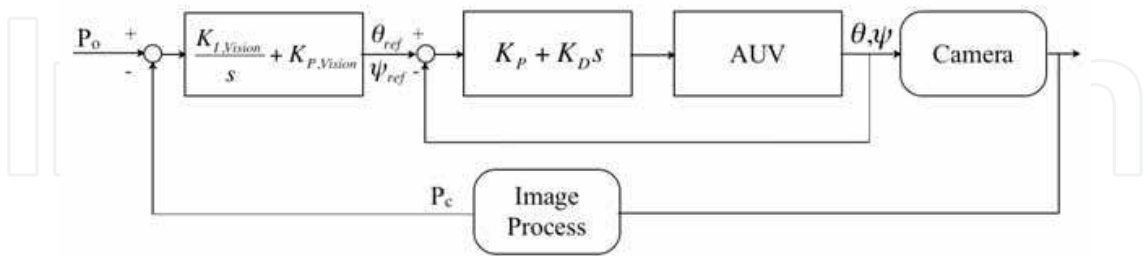
Fig. 21. The vision-guidance control algorithm. P_o is the origin of the image coordinate frame. P_c is the estimated center of the dock. \theta is pitch, \psi is yaw. \theta_{ref} and \psi_{ref} are generated reference pitch and yaw, respectively.
