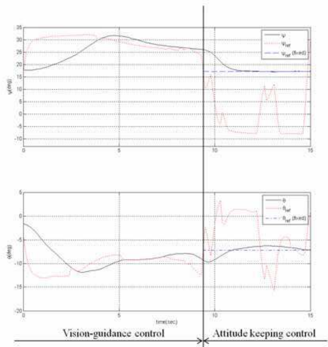
Fig. 26. Final approach: (upper) Yaw, Ref. yaw and fixed ref. yaw (lower) Pitch, Ref. pitch and fixed ref. pitch are shown respectively. After 9 seconds, ref. yaw and ref. pitch were fixed. (1) t = 0 -9seconds : The vision-guidance control was applied. In this interval, all 5 lights were in the viewing range of the camera. (2) t = 9 -15seconds : At t = 9.4 seconds, the attitude keeping control began and the references were fixed.
