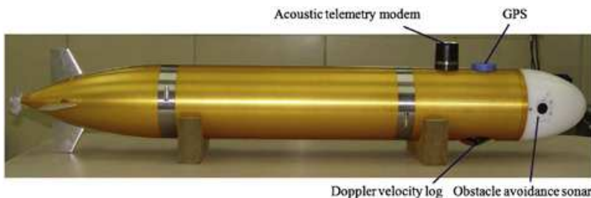
Figure 28. Sea-trial version of ISiMI AUV named ISiMI100
