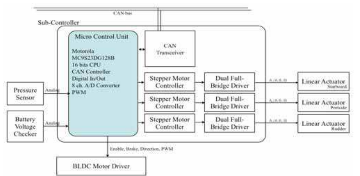
Fig. 5. Sub-controller.
