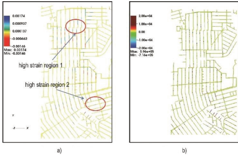
Figure 14. Distribution of strain and bending moment in part of pipeline network. (a) Normal strain; (b) bending moment.
