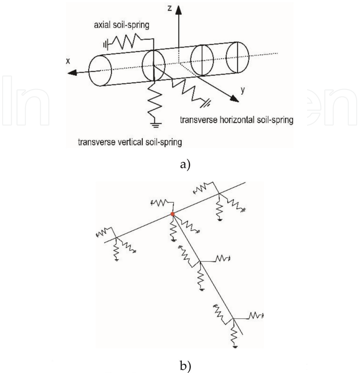
Figure 12. Soil-spring used in 1D line model: (a) shows three springs are attached to a pipe segment and (b) is a schematic view of a pipeline network attached with soil-springs.
