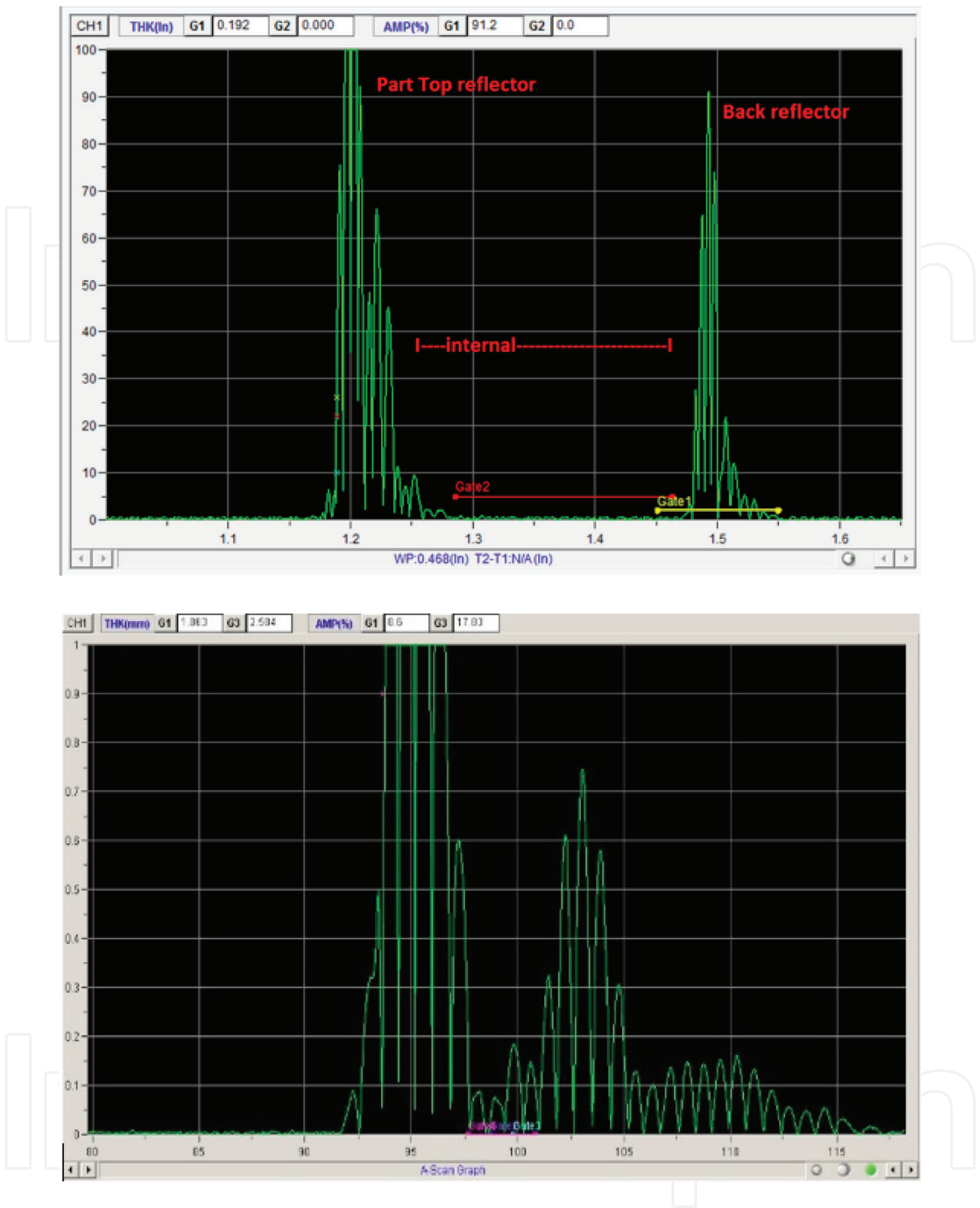
Figure 3. Upper: ultrasonic A-scan plot of the referenced autoclave cured composite laminates: void content <1%. Lower: the A-scan result of a COSB, indicating greater signal attenuation compared to the referenced laminate: void content ~6%.
