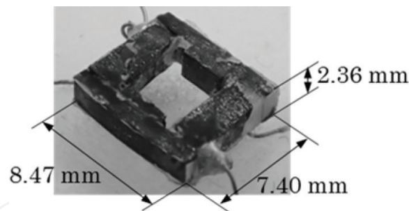
Figure 15. Fabricated multilayer ceramic magnetic circuit.
