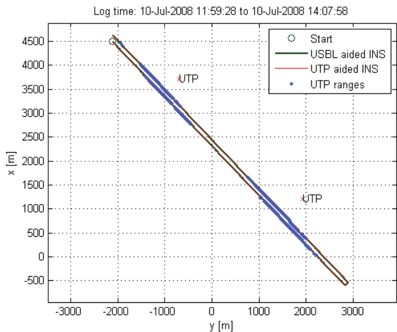
Fig. 6. North (x) and east (y) relative coordinates of 2D AUV trajectory during sea trial. Two UTP transponders were deployed 4 km apart.
