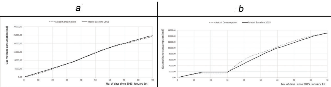
Figure 7. Comparison between cumulative simulated and measured consumption at the community clinic in 2013 (a) and 2015 (b).
