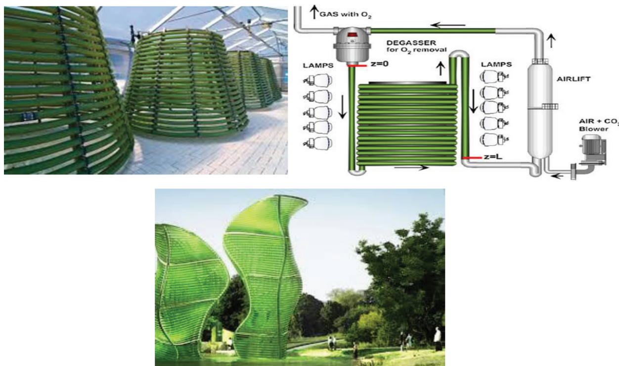
Figure 2. Helical photobioreactor.
