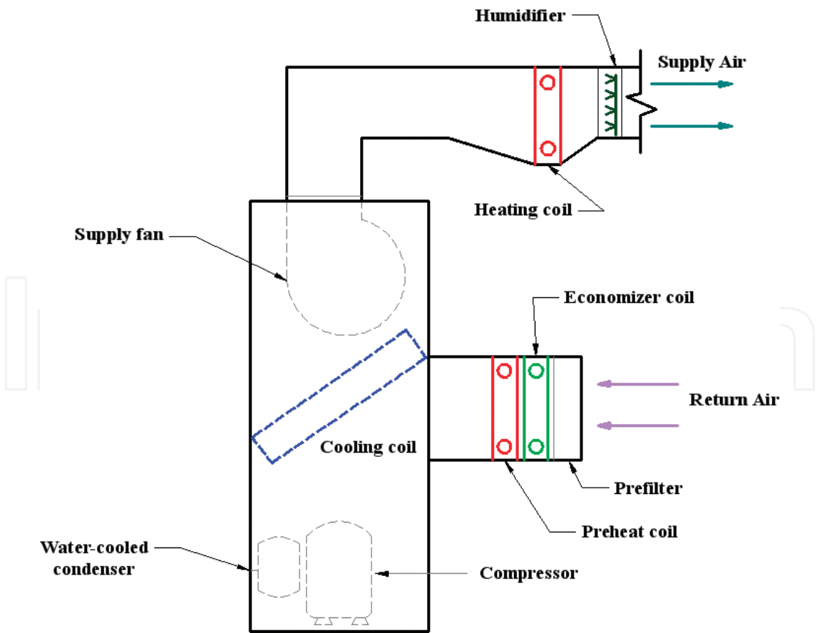
Figure 13. Unitary air-conditioner package.
