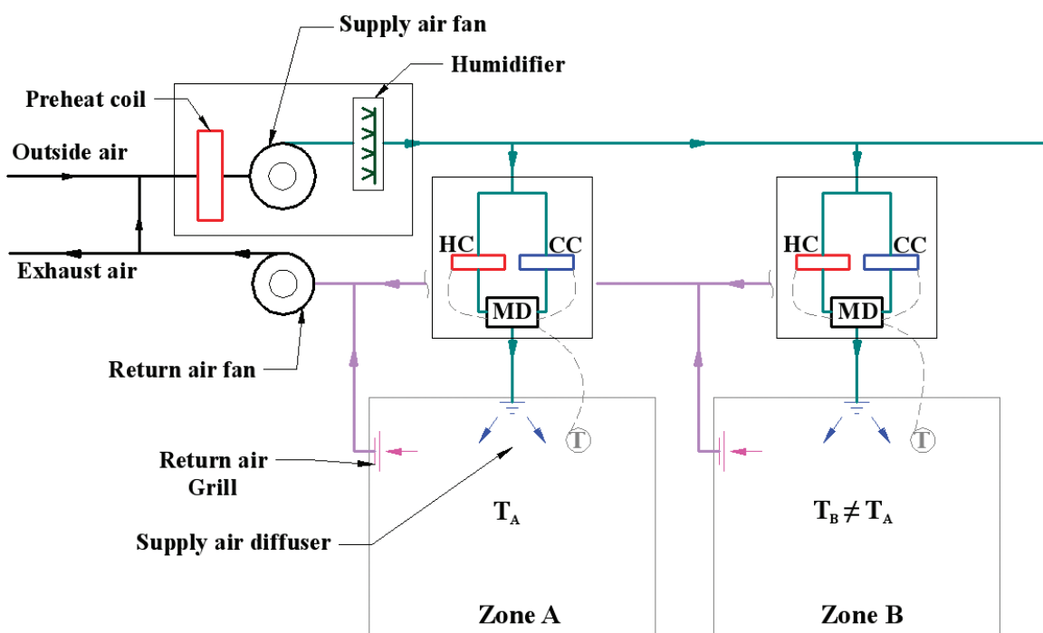
Figure 5. All-air HVAC system for multiple zones.
