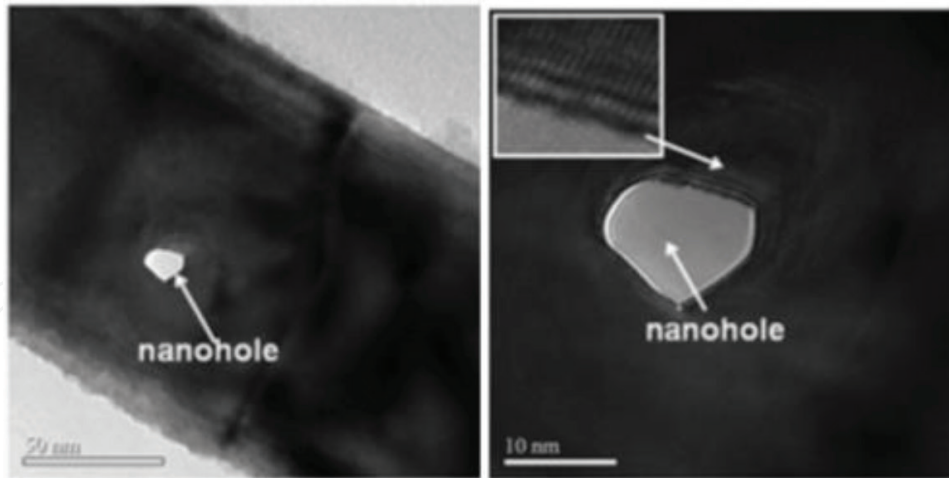
Figure 1. Focused electron beam to create nanoholes in ZnO nanowires [1].
