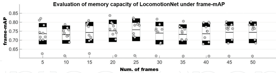
Figure 9. Memory capacity in MHI for the locomotion level of the multilevel action descriptor.
