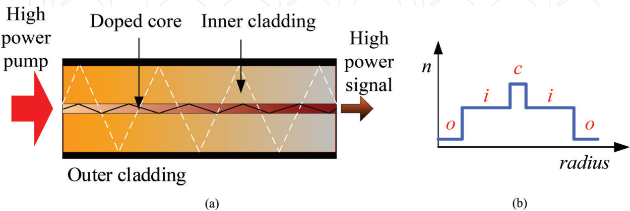
Figure 2. (a) The double-clad fiber concept of high power fiber lasers. (b) Refractive index profile. c: core, i: inner cladding, o: outer cladding.
