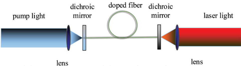
Figure 1. A schematic setup of a basic fiber laser.
