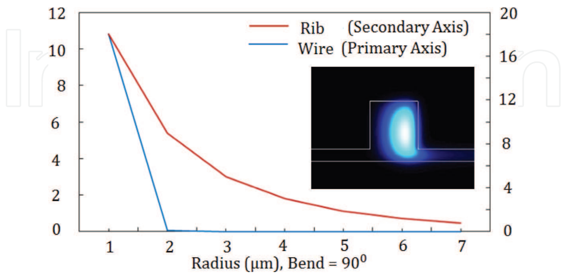
Figure 13. Mode loss for silicon wire (cross-section: 450 \times 220 \text{ nm}^2 ) and rib (cross-section: 600 \times 220 \text{ nm}^2 ) waveguides for a 90° bend with increasing bending radii.
