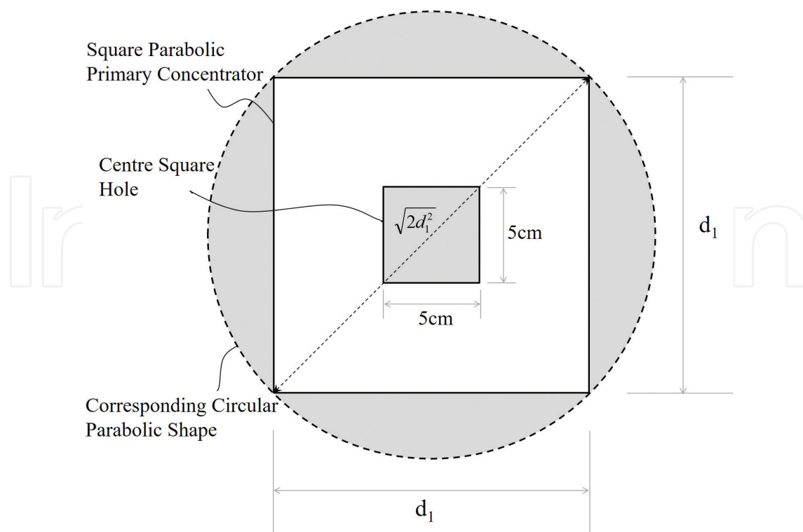
Figure 3. Simple schematic for primary reflector size calculations.
