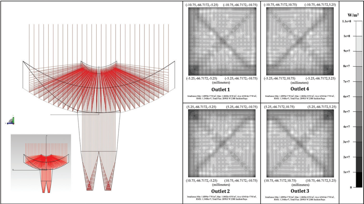
Figure 9. Ray tracing simulation of multicell concentrating assembly for parallel rays.
