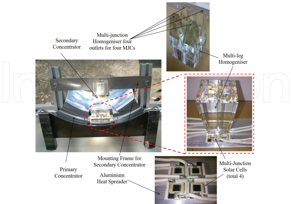
Figure 6. Developed prototype of multicell concentrating assembly (MCA)-based CPV module.
