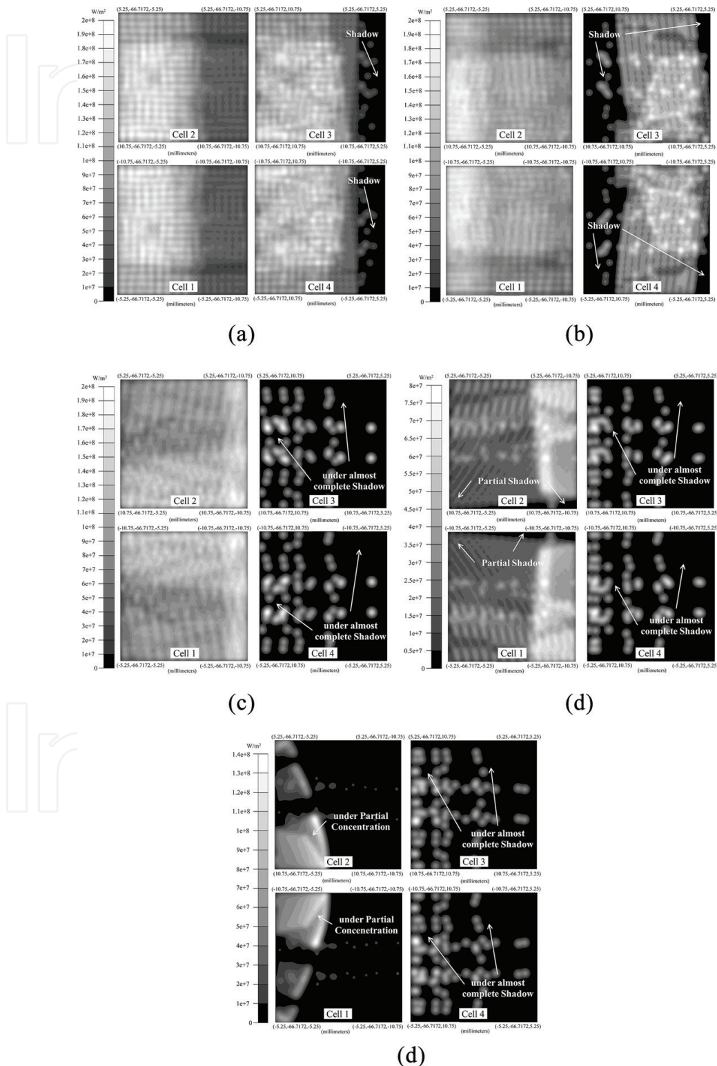
Figure 14. Simulated irradiance map at outlet apertures of multi-leg homogenizer for different angular deviations of parallel rays.
