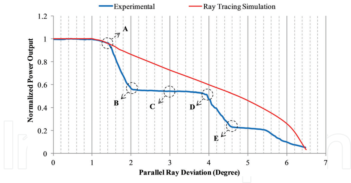
Figure 13. Normalized power curves for multicell concentrating assembly-based CPV system.
