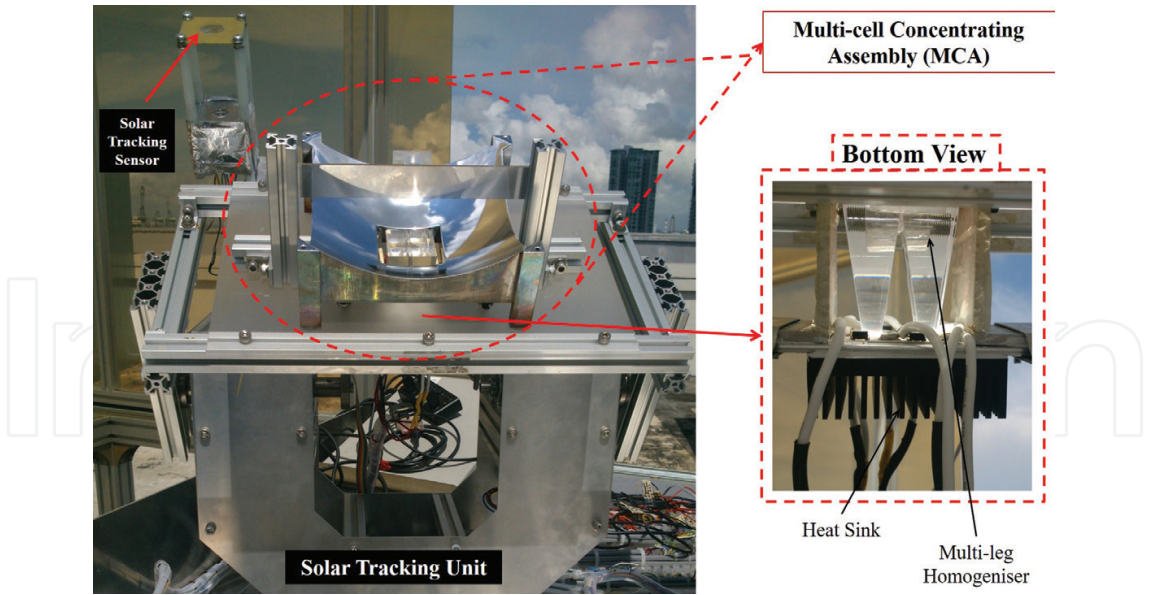
Figure 7. Experimental prototype of MCA-based novel CPV unit.
