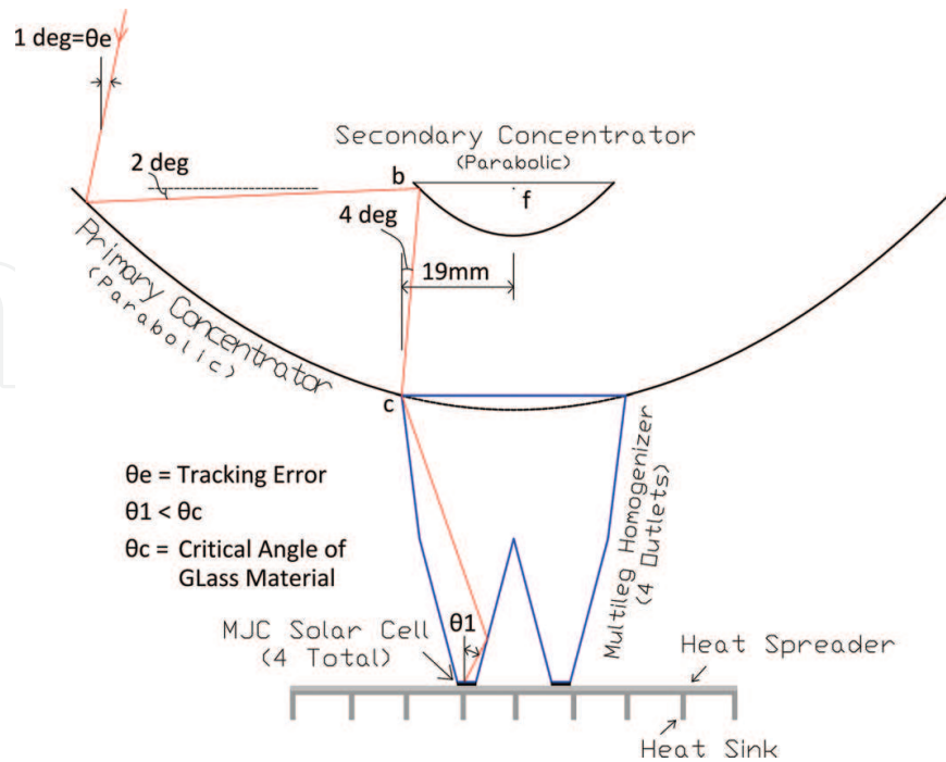
Figure 5. Acceptance angle calculation for multicell concentrating assembly.
