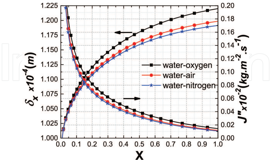
Figure 13. Effect of the type of non-condensable gas on the evolution of the liquid film thickness and the condensing mass flux at the interface along the tube.
