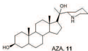
Figure 3. General structures of inhibitors of 24-SMT.
